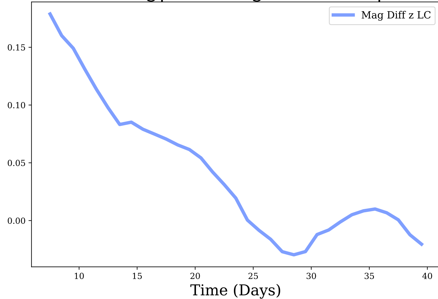
z-band, Avg|Max Mag Diff: 0.04 | 0.18
