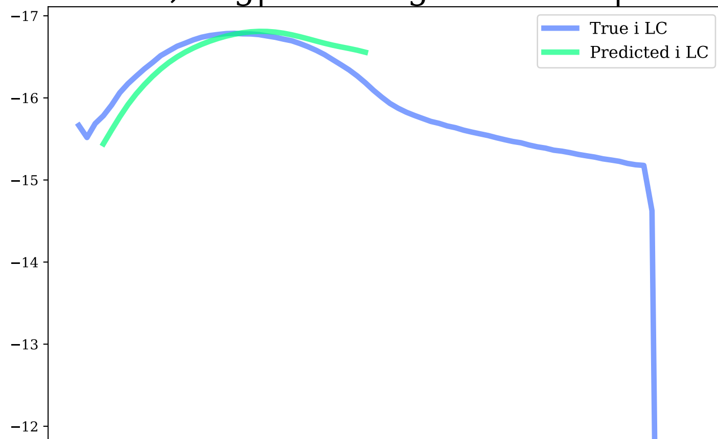
i-band, Avg|Max Mag Diff: 0.14 | 0.37
