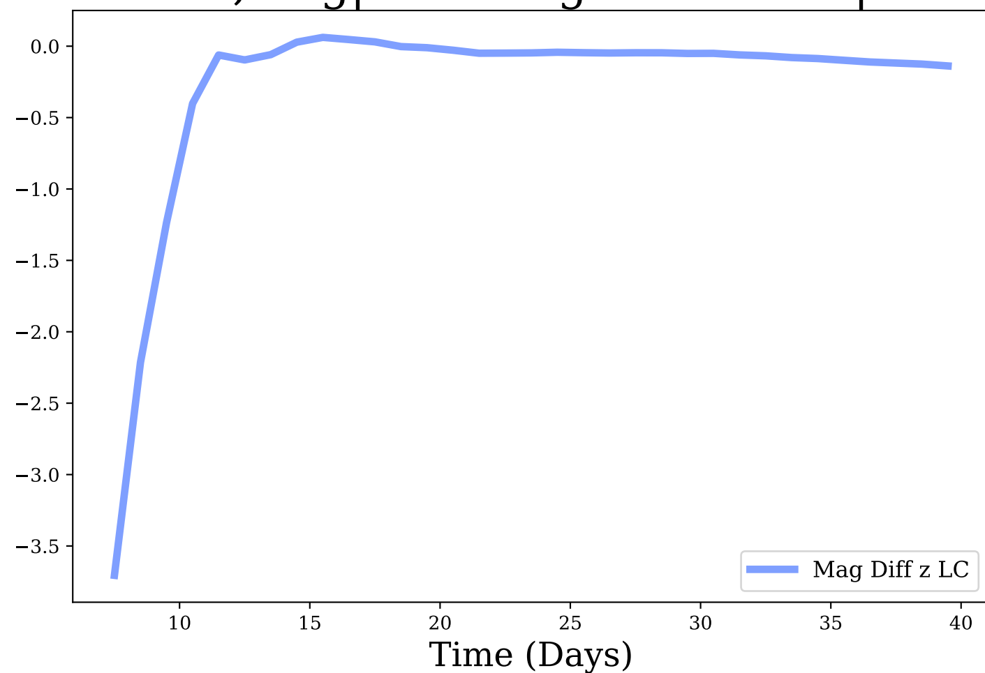
z-band, Avg|Max Mag Diff: -0.27 | 3.71
