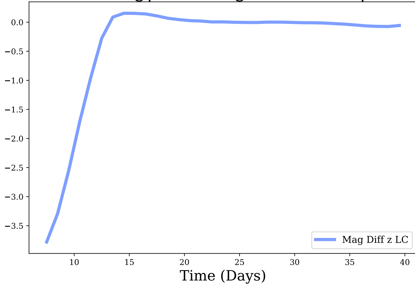
z-band, Avg|Max Mag Diff: -0.37 | 3.78
