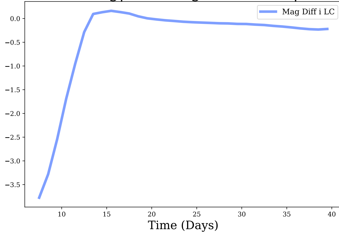
i-band, Avg|Max Mag Diff: -0.44 | 3.78
