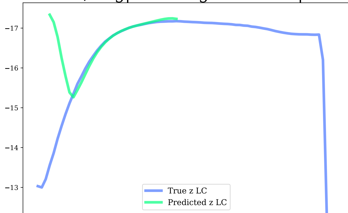
z-band, Avg|Max Mag Diff: 0.42 | 3.78
