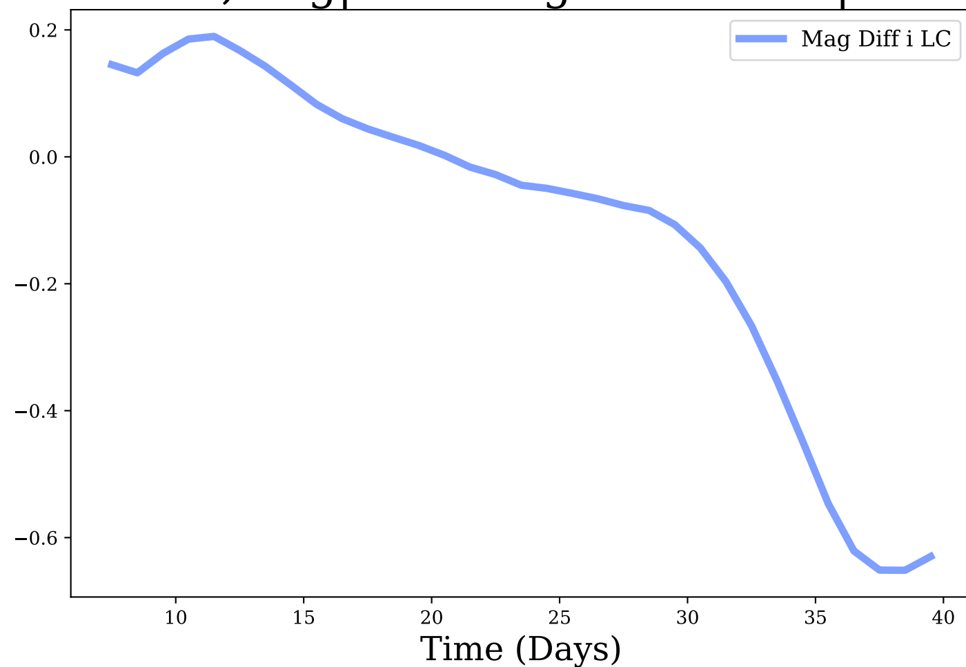
i-band, Avg|Max Mag Diff: -0.11 | 0.65
