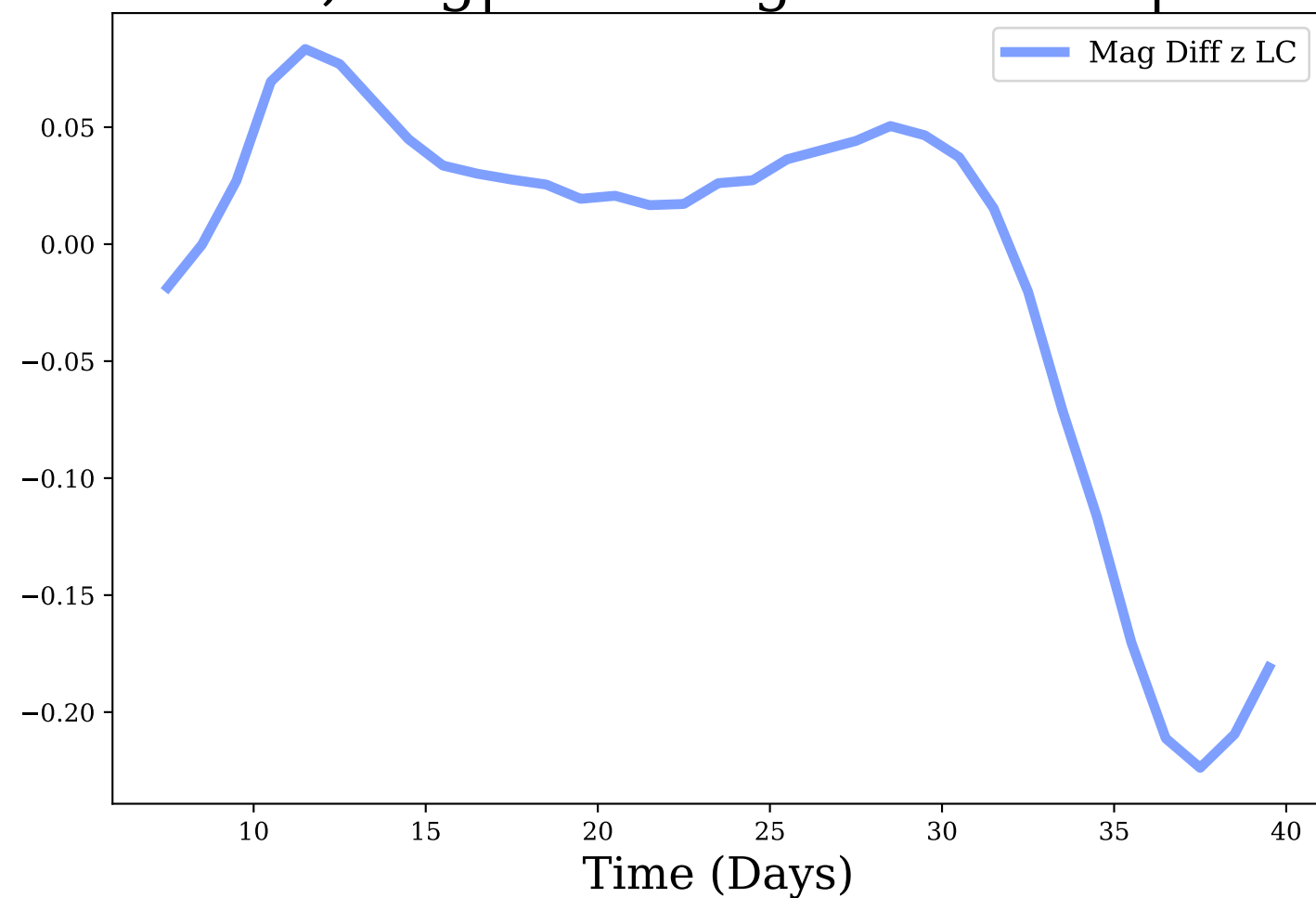
z-band, Avg|Max Mag Diff: -0.01 | 0.22
