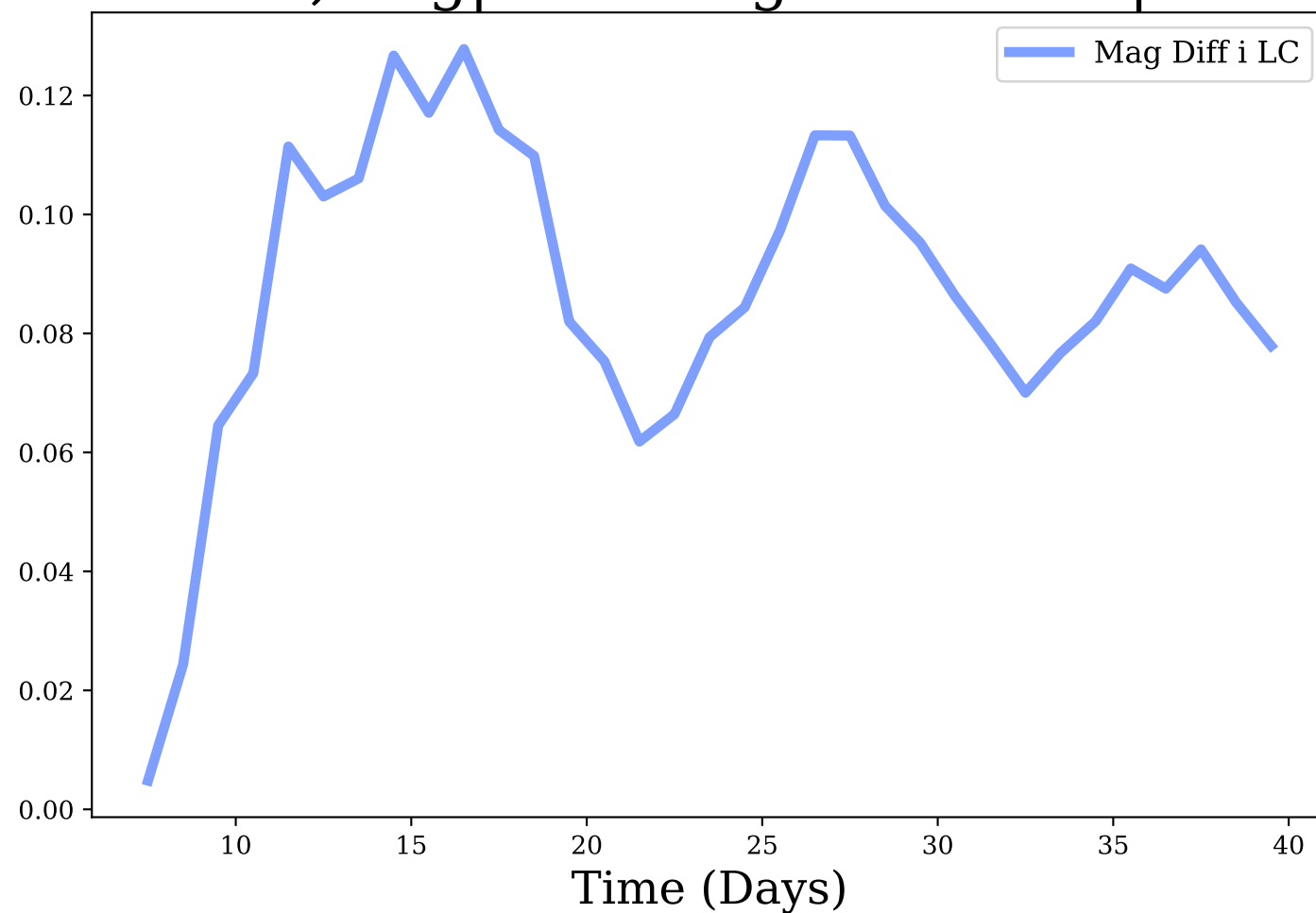
i-band, Avg|Max Mag Diff: 0.09 | 0.13
