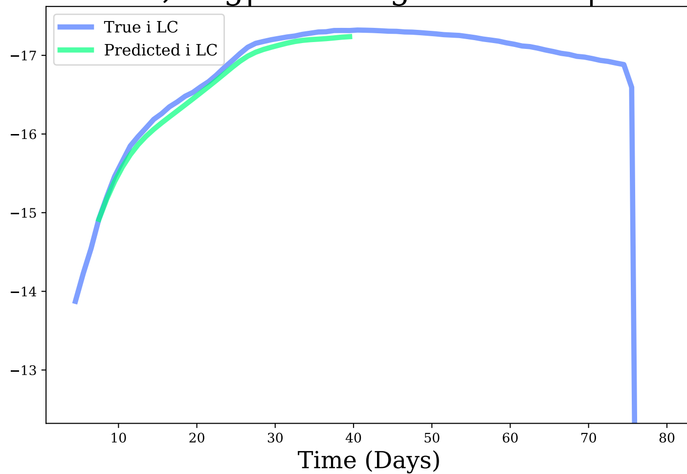
i-band, Avg|Max Mag Diff: 0.09 | 0.13
