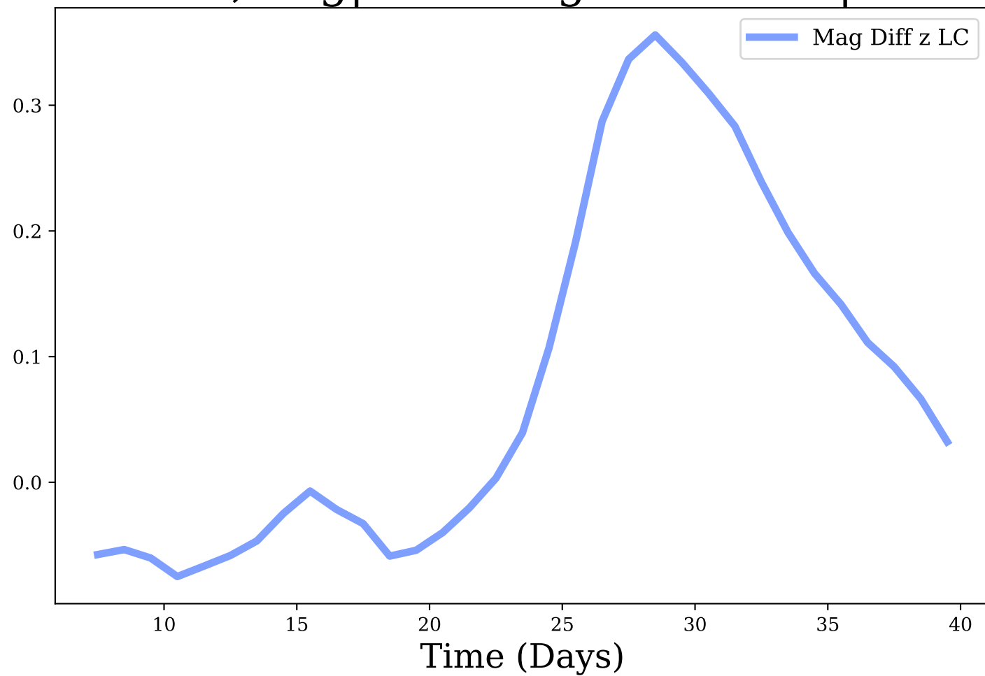
z-band, Avg|Max Mag Diff: 0.08 | 0.36
