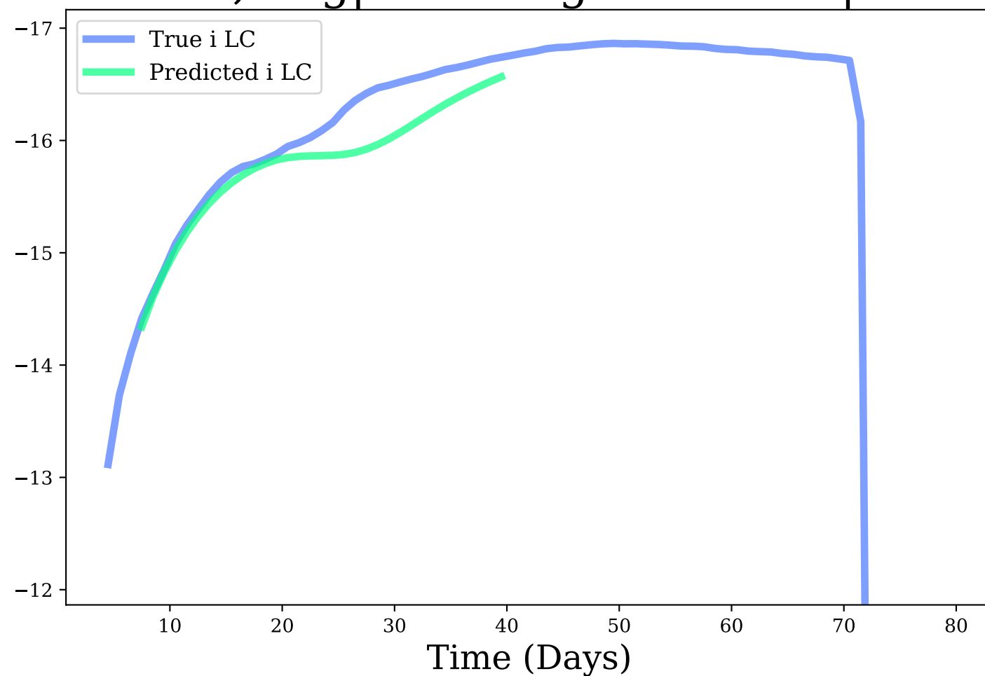
i-band, Avg|Max Mag Diff: 0.21 | 0.51
