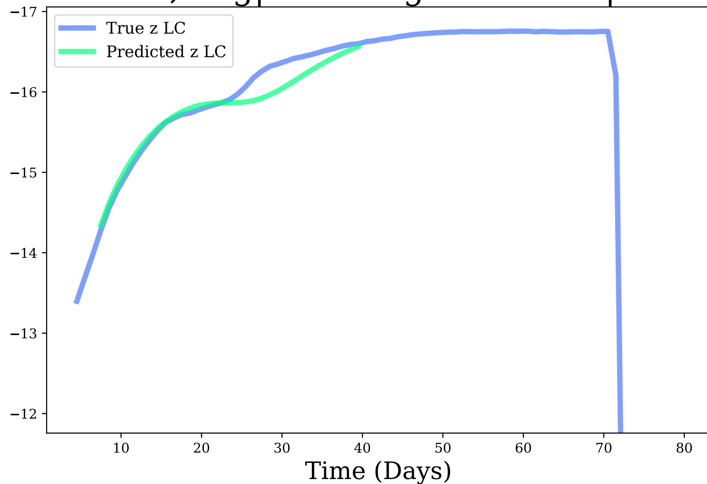
z-band, Avg|Max Mag Diff: 0.12 | 0.36
