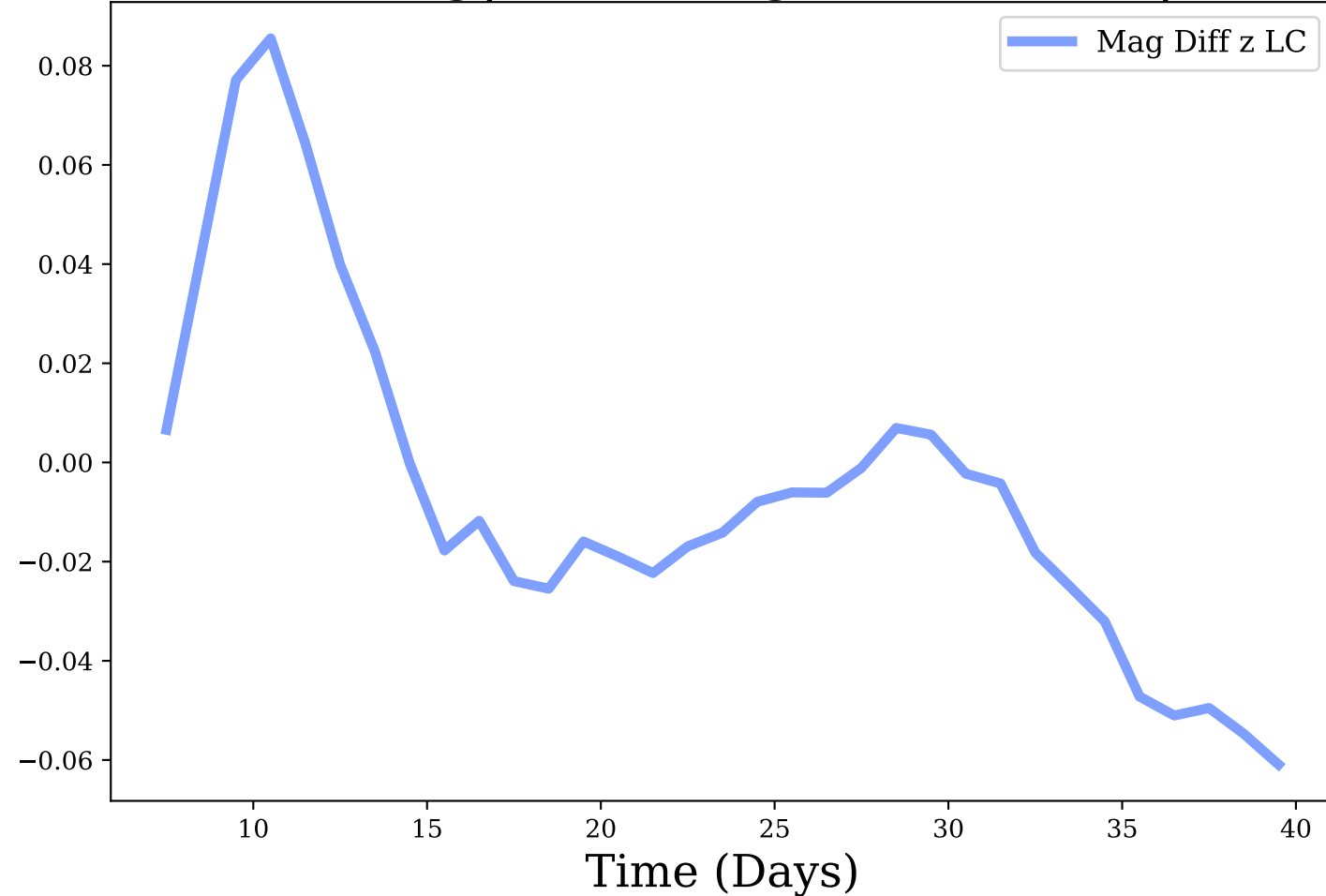
z-band, Avg|Max Mag Diff: -0.01 | 0.09
