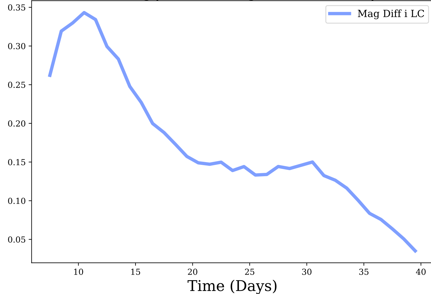
i-band, Avg|Max Mag Diff: 0.17 | 0.34
