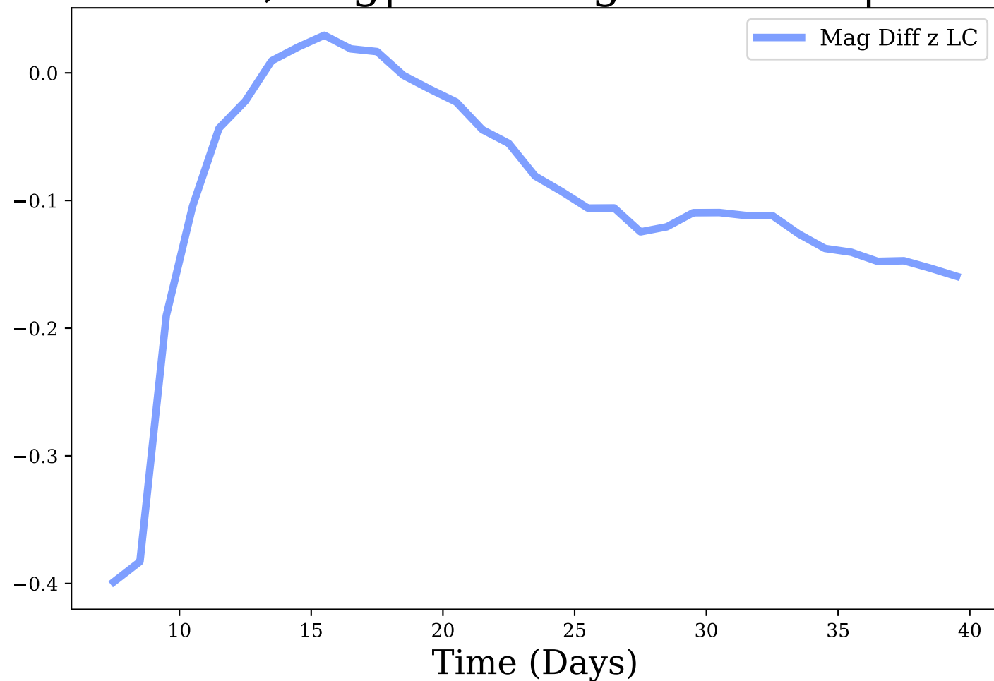
z-band, Avg|Max Mag Diff: -0.1 | 0.4
