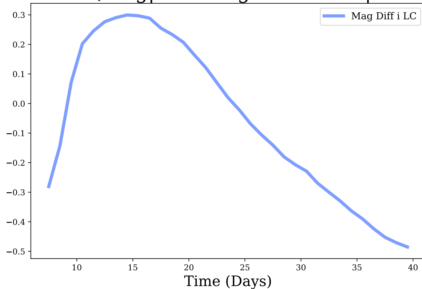
i-band, Avg|Max Mag Diff: -0.06 | 0.49
