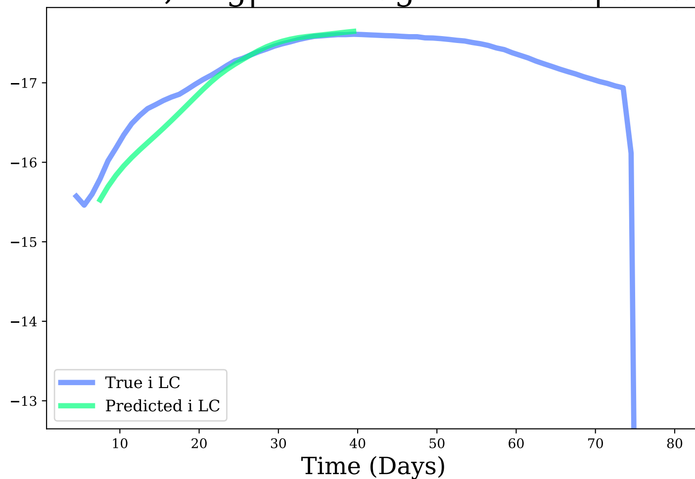
i-band, Avg|Max Mag Diff: 0.15 | 0.43
