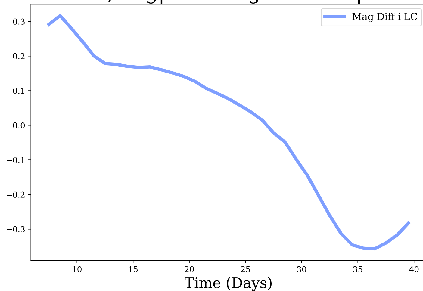
i-band, Avg|Max Mag Diff: 0.0 | 0.36
