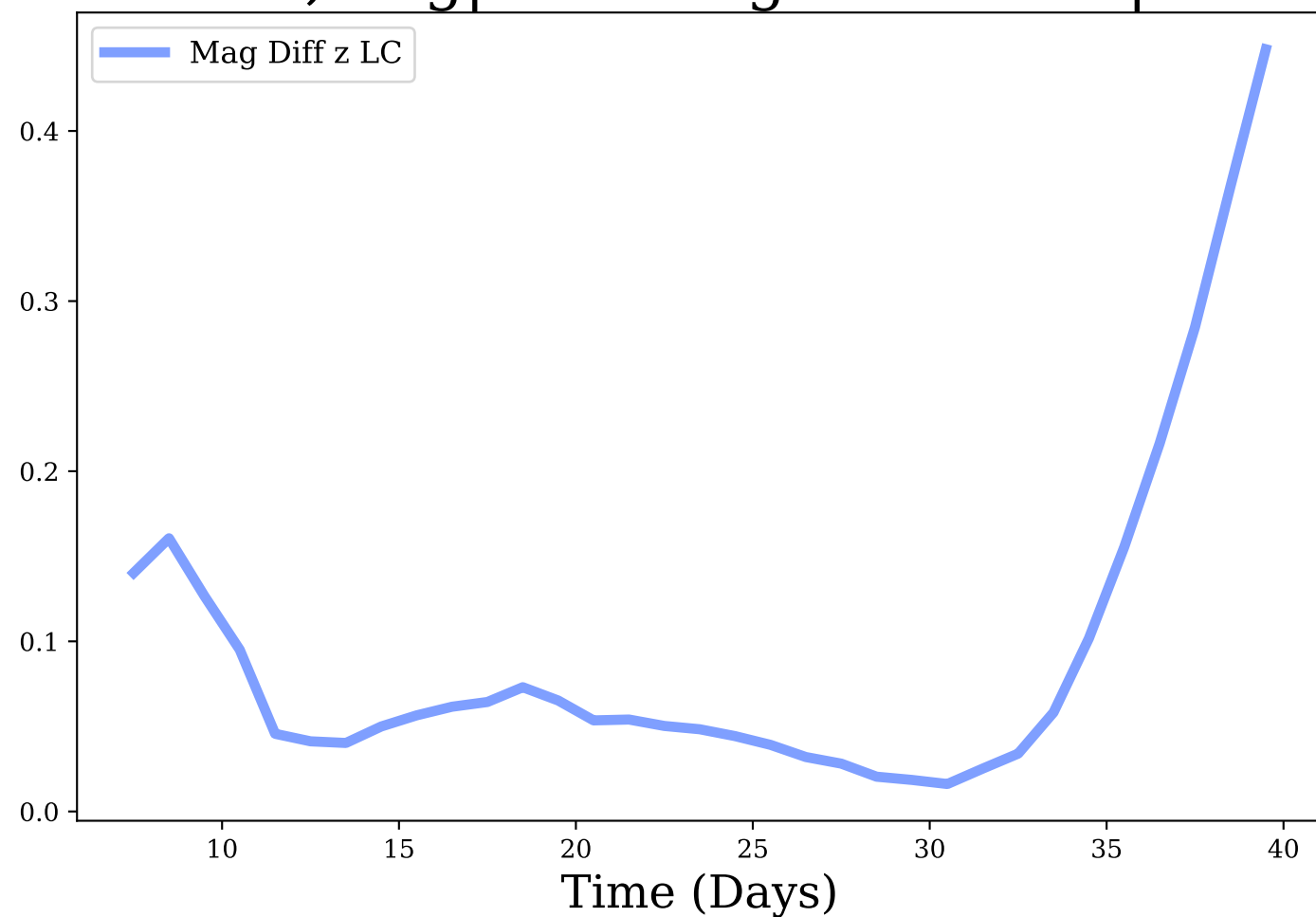
z-band, Avg|Max Mag Diff: 0.09 | 0.45
