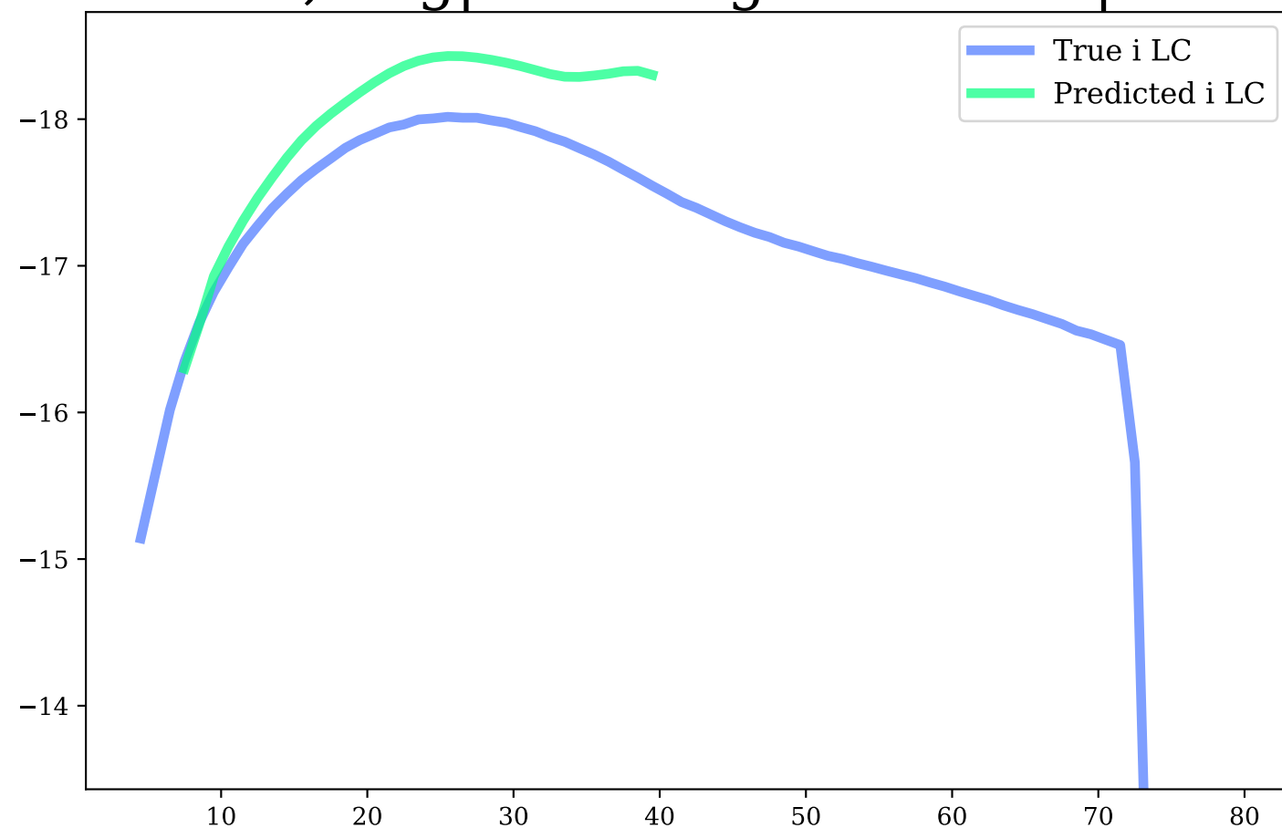
i-band, Avg|Max Mag Diff: 0.37 | 0.76
