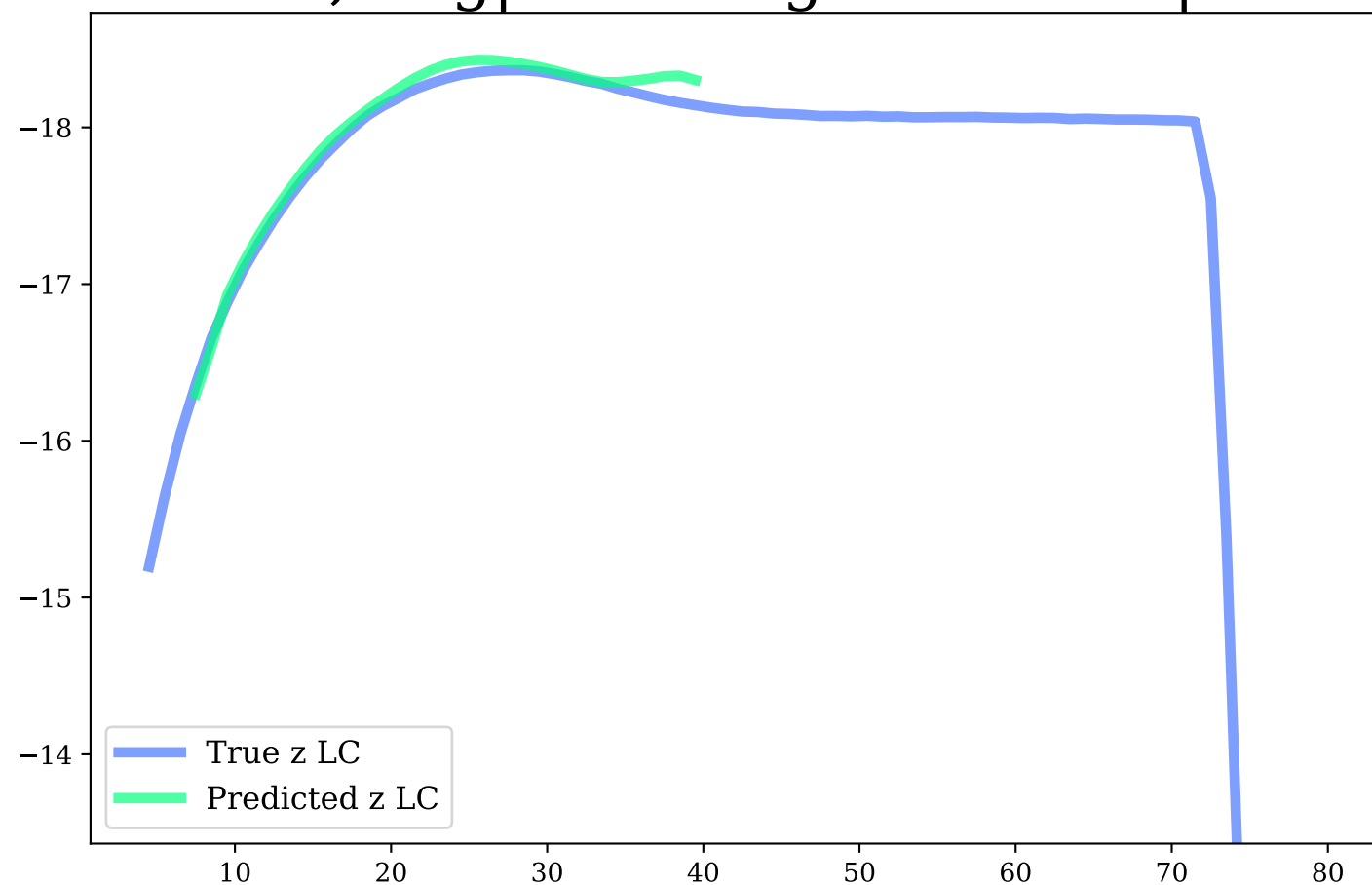
z-band, Avg|Max Mag Diff: 0.06 | 0.17
