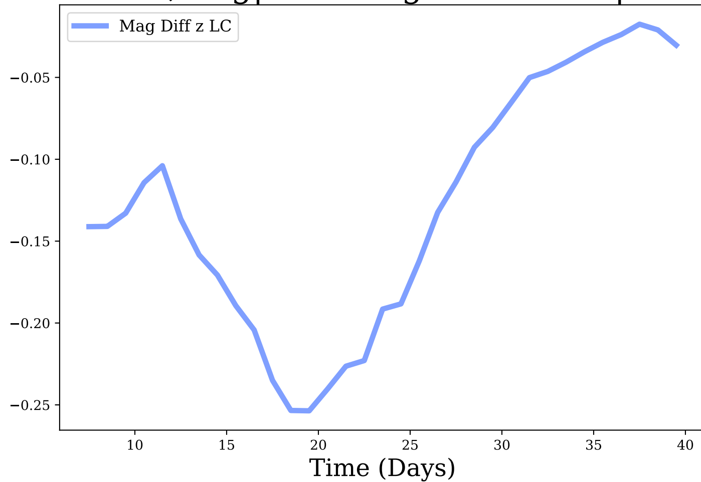
z-band, Avg|Max Mag Diff: -0.13 | 0.25
