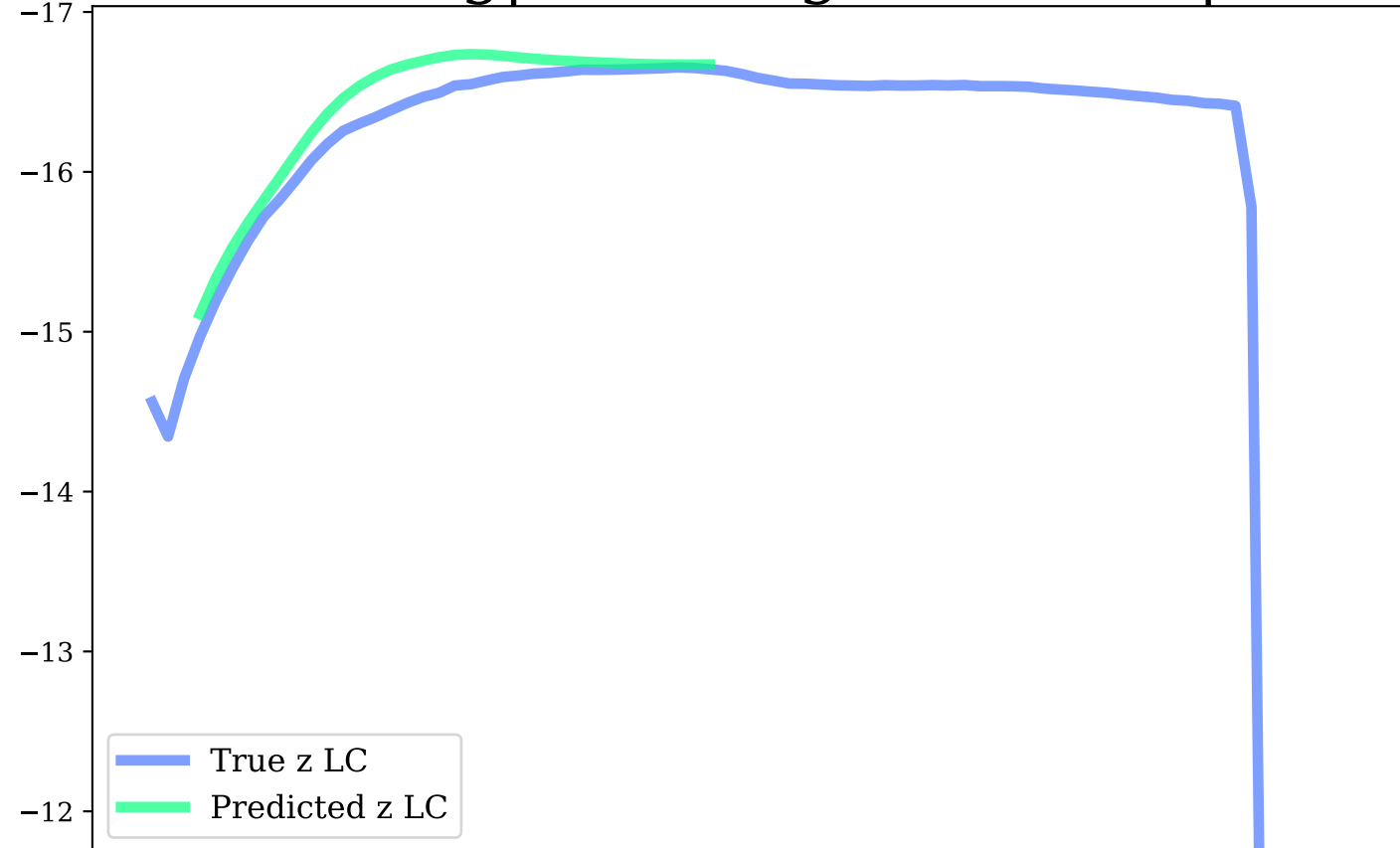
z-band, Avg|Max Mag Diff: 0.13 | 0.25
