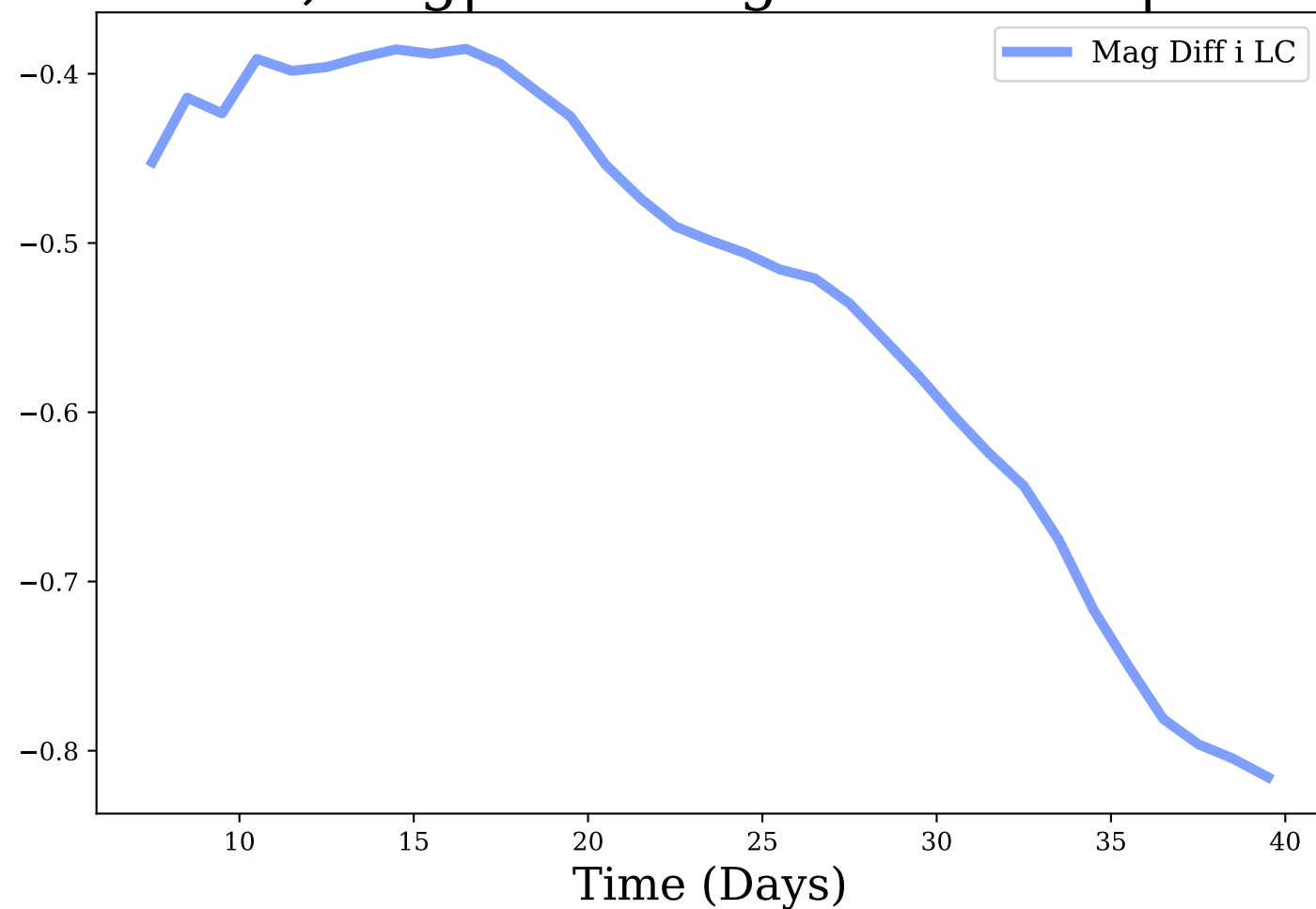
i-band, Avg|Max Mag Diff: -0.53 | 0.82
