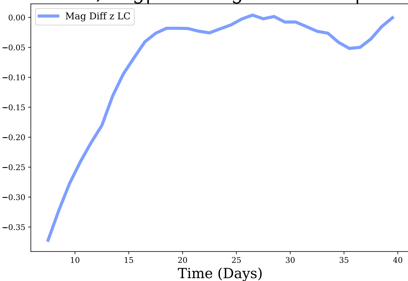
z-band, Avg|Max Mag Diff: -0.07 | 0.37
