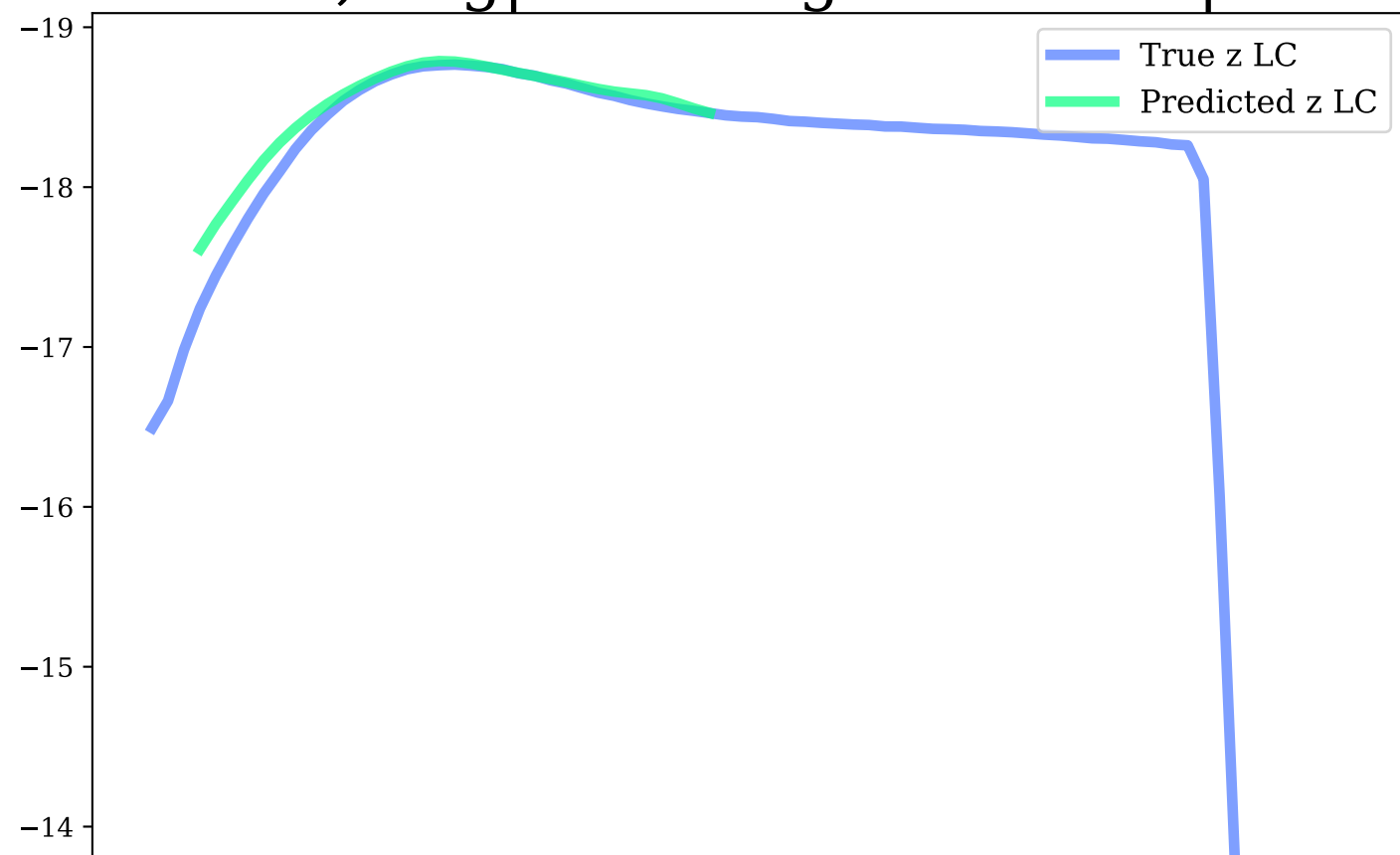
z-band, Avg|Max Mag Diff: 0.07 | 0.37
