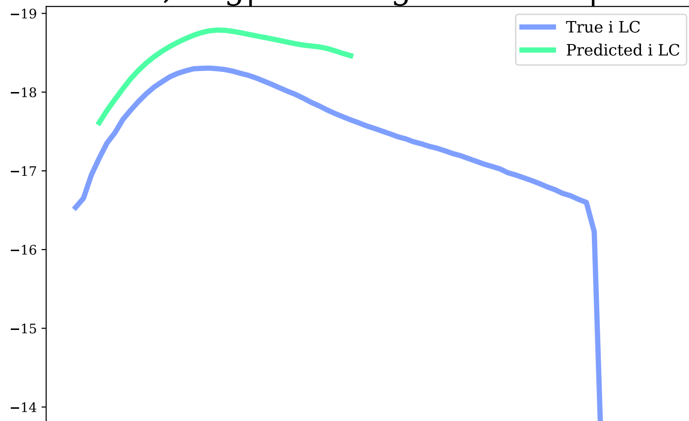
i-band, Avg|Max Mag Diff: 0.53 | 0.82
