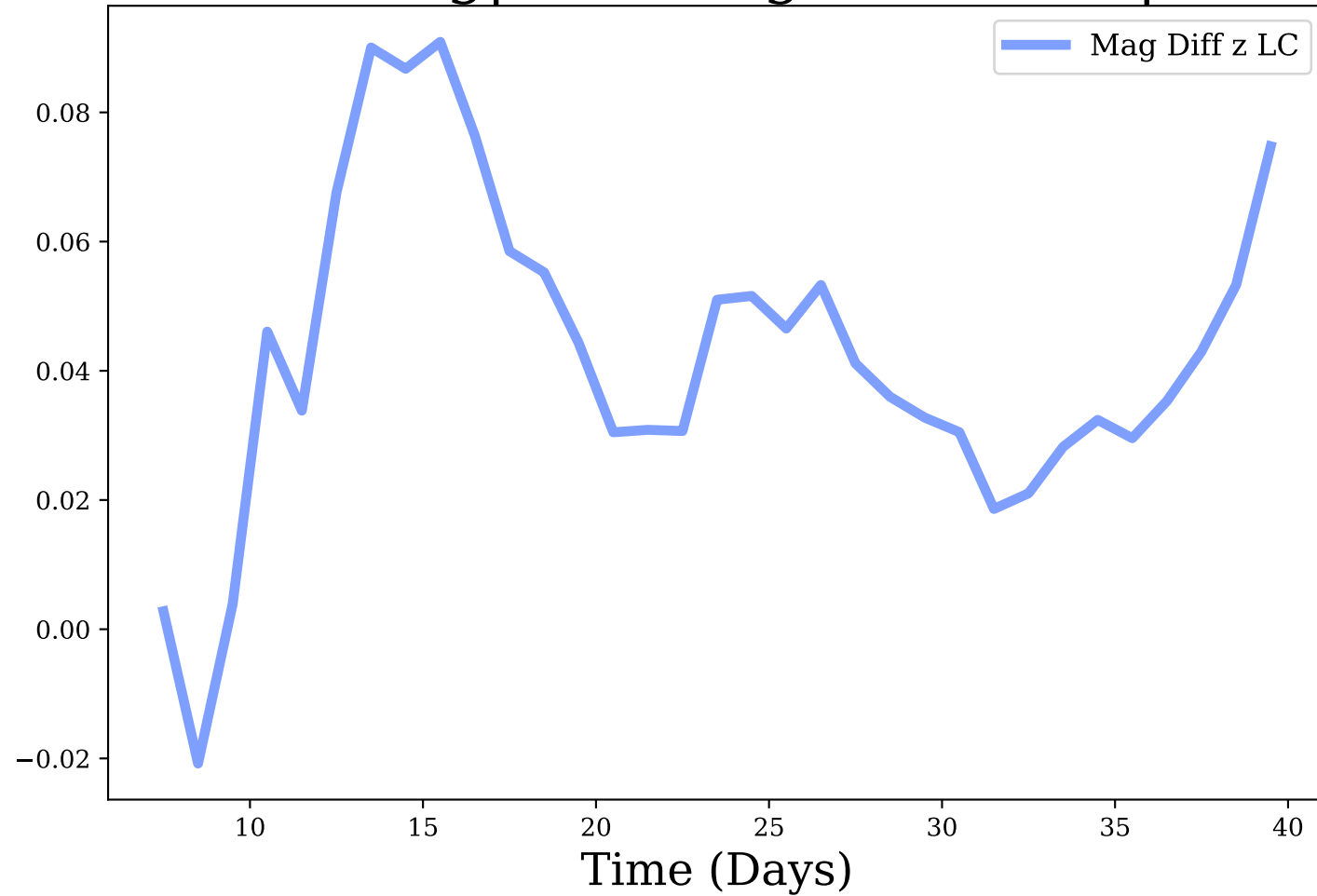
z-band, Avg|Max Mag Diff: 0.04 | 0.09
