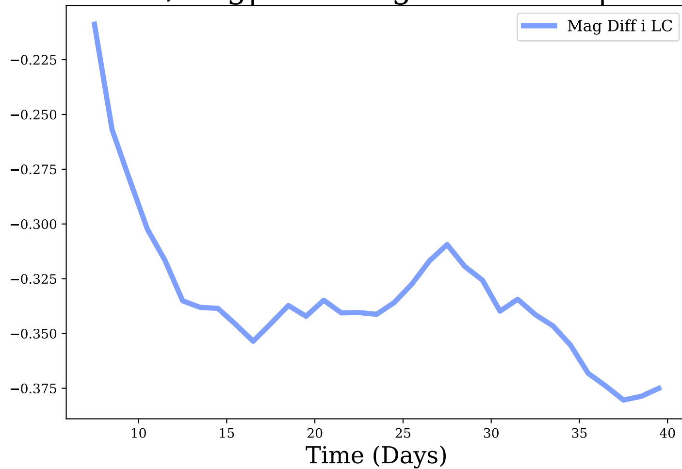
i-band, Avg|Max Mag Diff: -0.33 | 0.38
