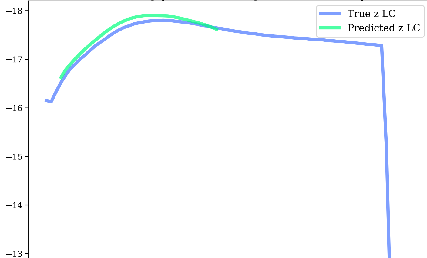
z-band, Avg|Max Mag Diff: 0.1 | 0.14
