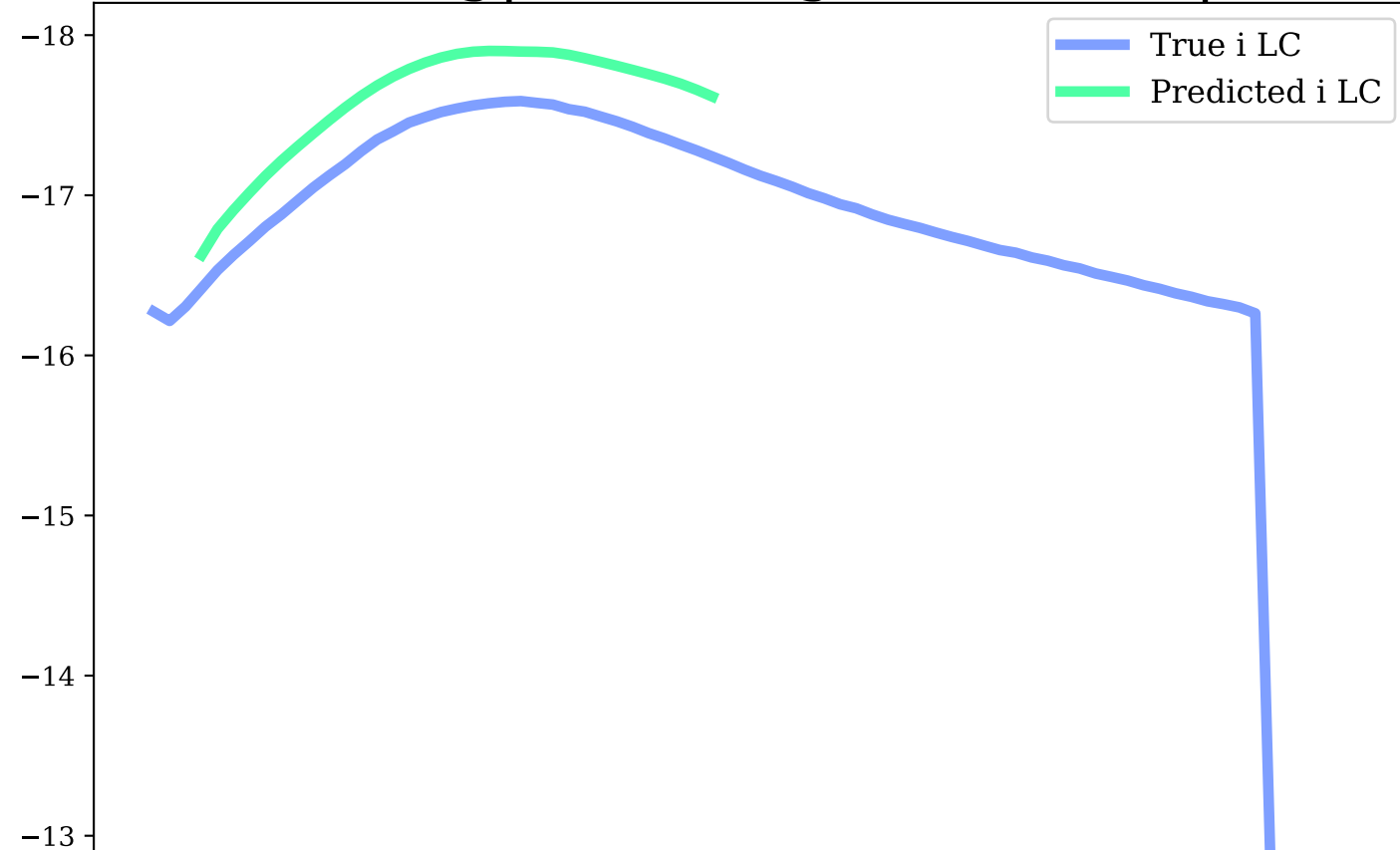
i-band, Avg|Max Mag Diff: 0.33 | 0.38
