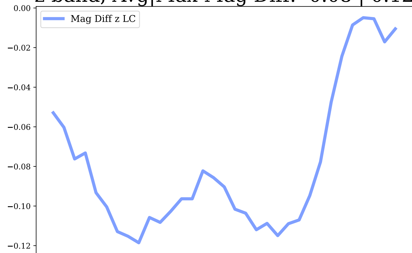
z-band, Avg|Max Mag Diff: -0.08 | 0.12
