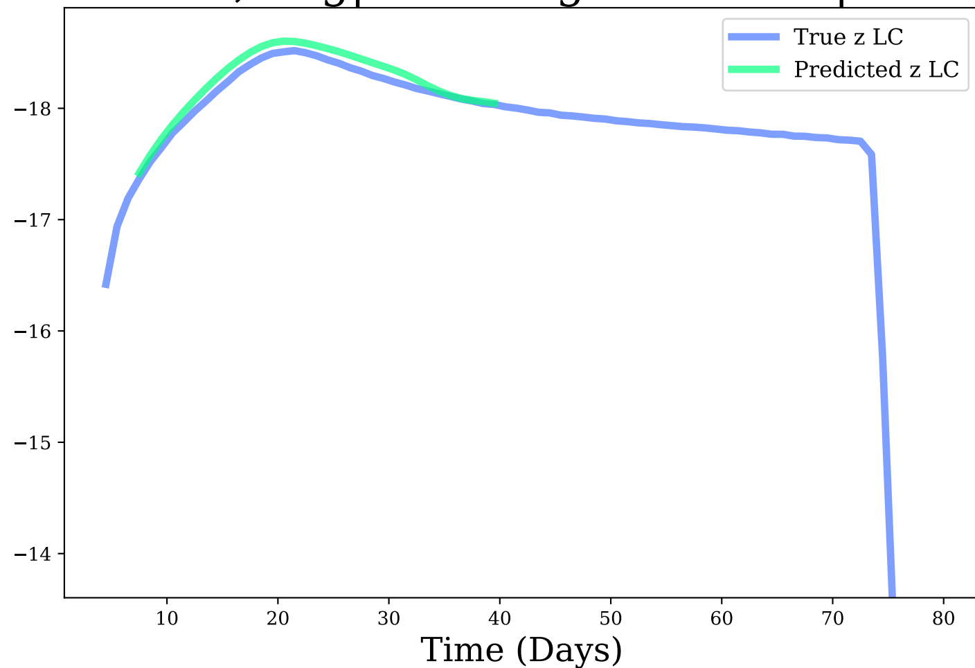
z-band, Avg|Max Mag Diff: 0.08 | 0.12
