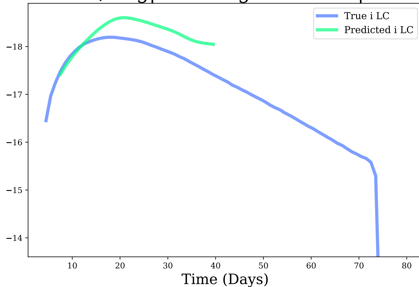
i-band, Avg|Max Mag Diff: 0.35 | 0.63
