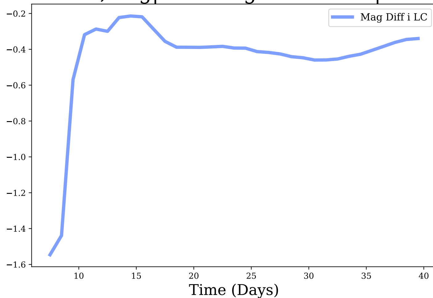
i-band, Avg|Max Mag Diff: -0.45 | 1.55
