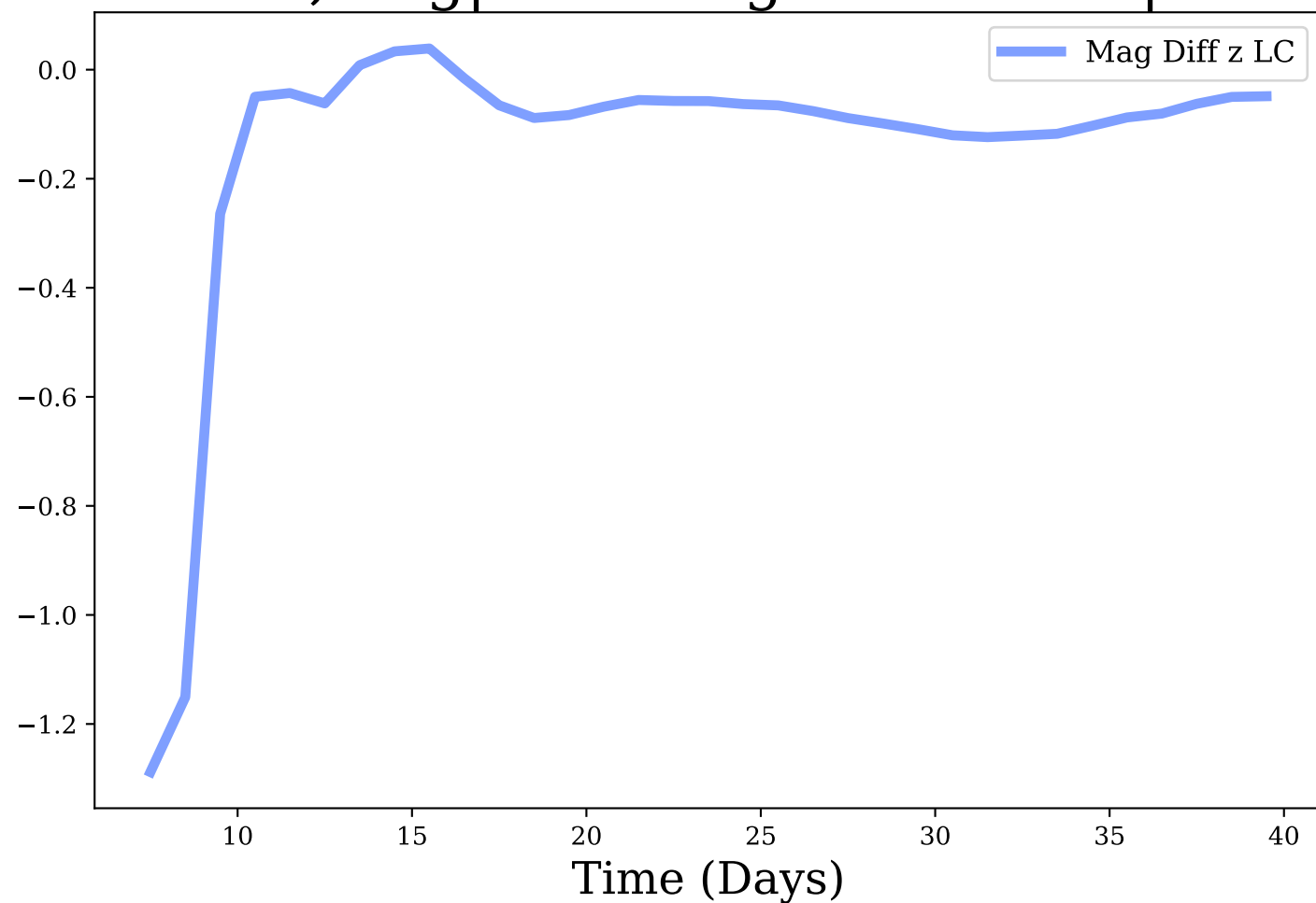
z-band, Avg|Max Mag Diff: -0.14 | 1.29
