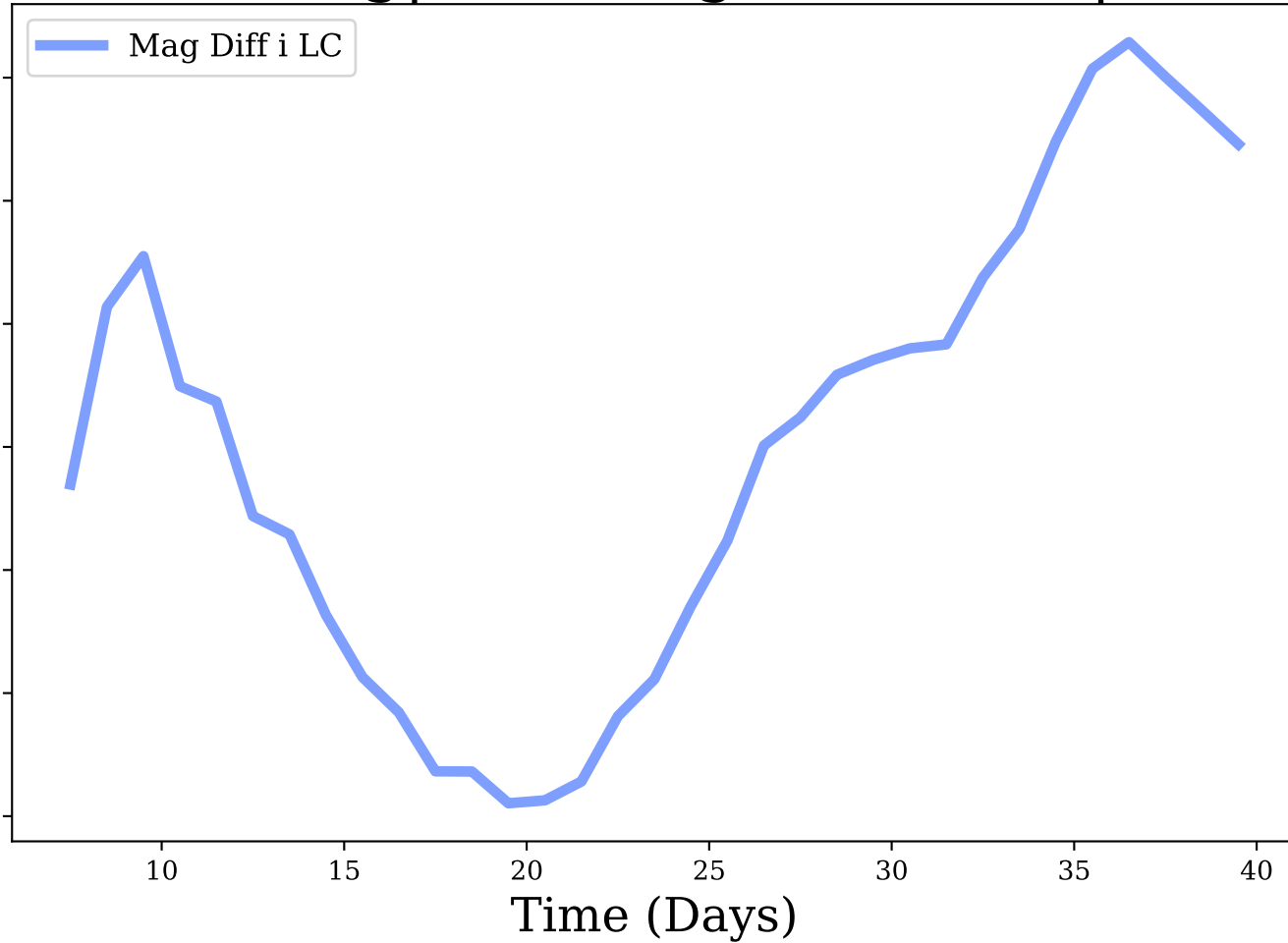
i-band, Avg|Max Mag Diff: 0.15 | 0.31
