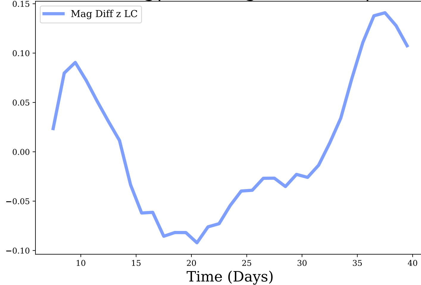
z-band, Avg|Max Mag Diff: 0.01 | 0.14
