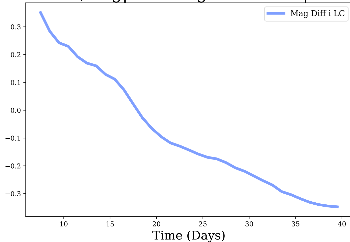
i-band, Avg|Max Mag Diff: -0.08 | 0.35
