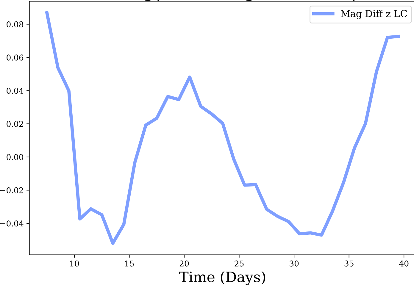
z-band, Avg|Max Mag Diff: 0.0 | 0.09
