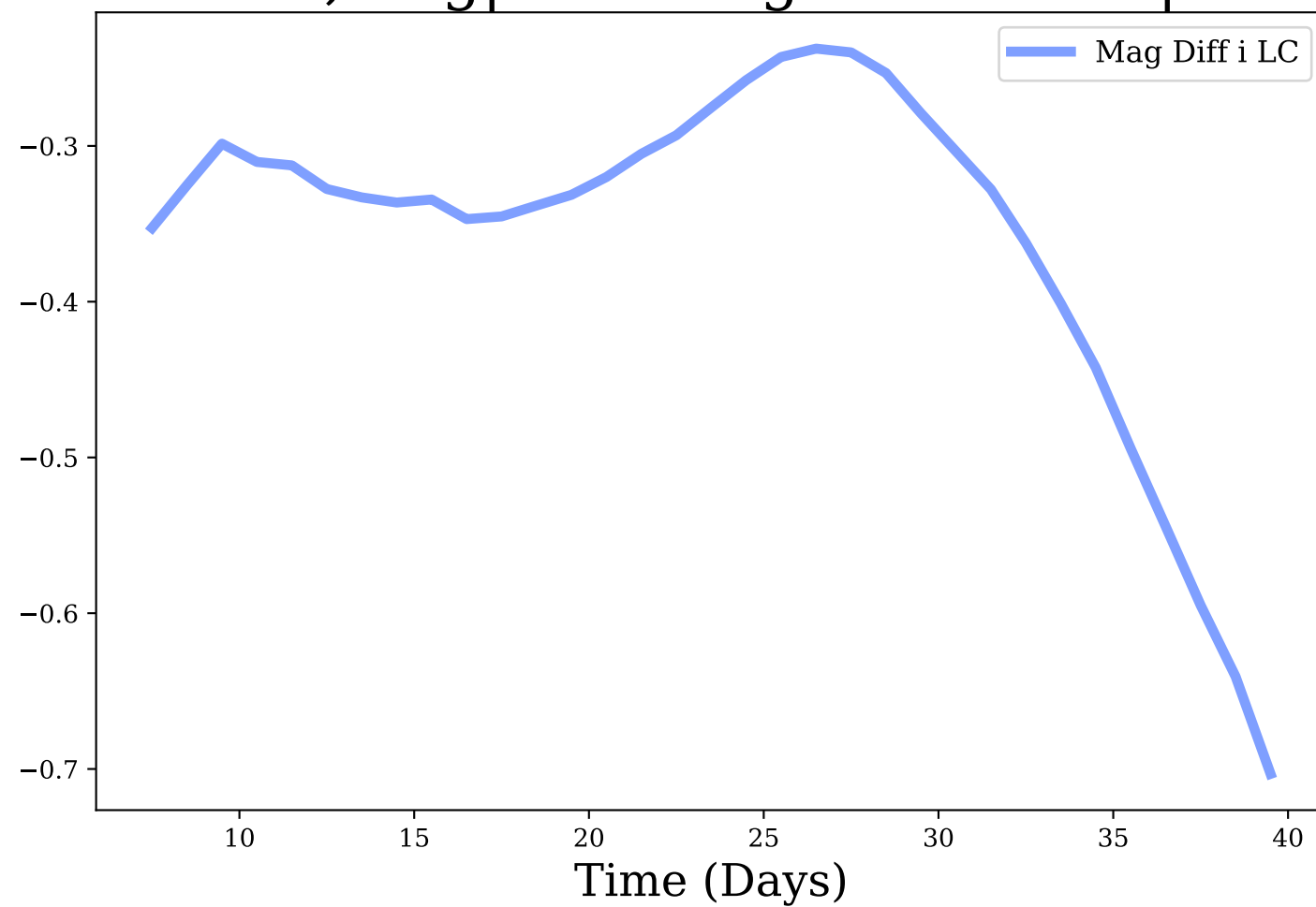
i-band, Avg|Max Mag Diff: -0.36 | 0.7
