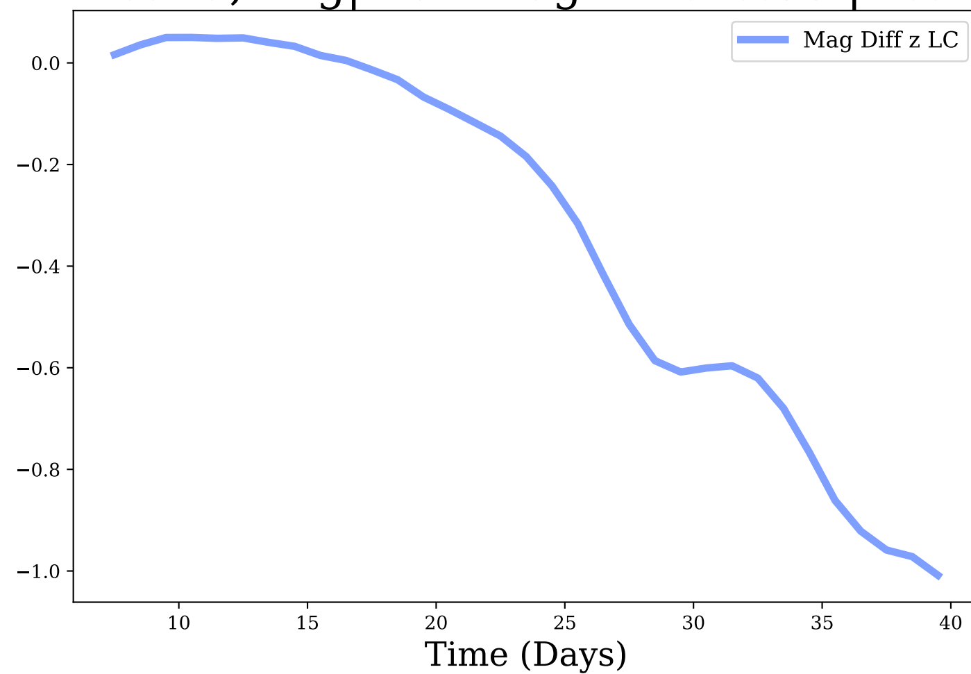
z-band, Avg|Max Mag Diff: -0.33 | 1.01
