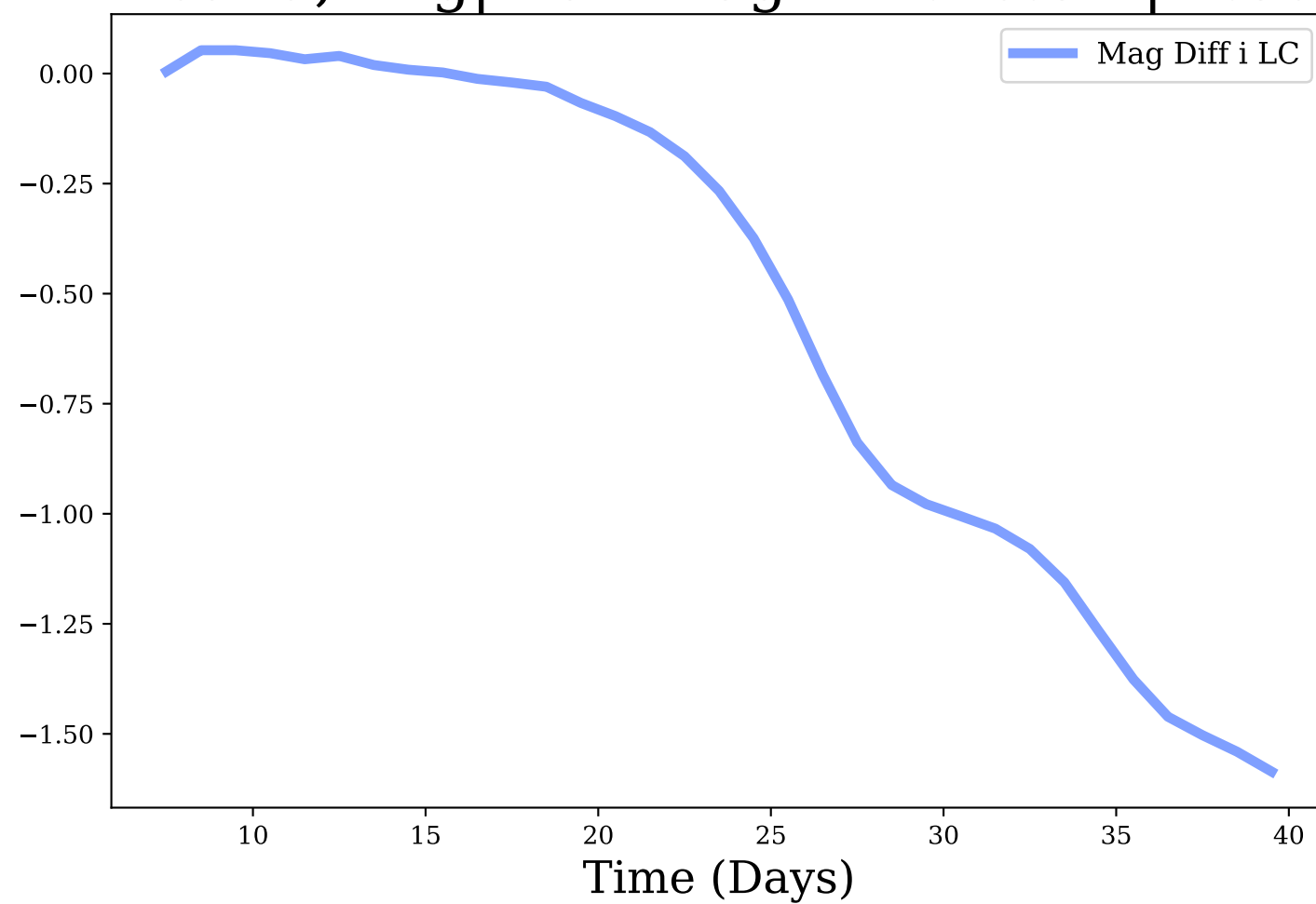
i-band, Avg|Max Mag Diff: -0.54 | 1.59
