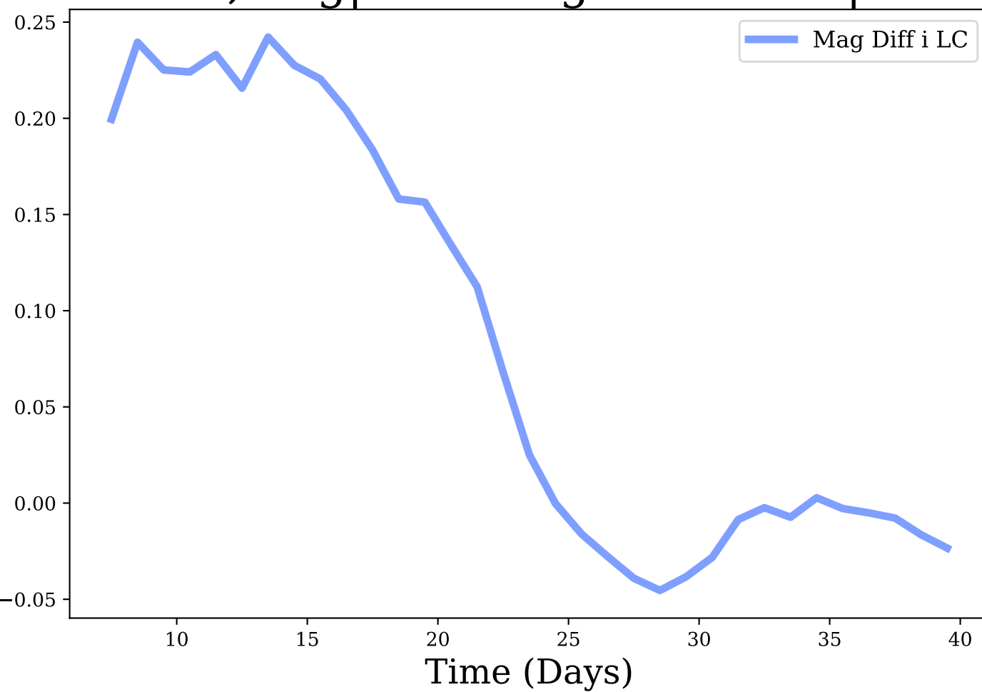
i-band, Avg|Max Mag Diff: 0.08 | 0.24
