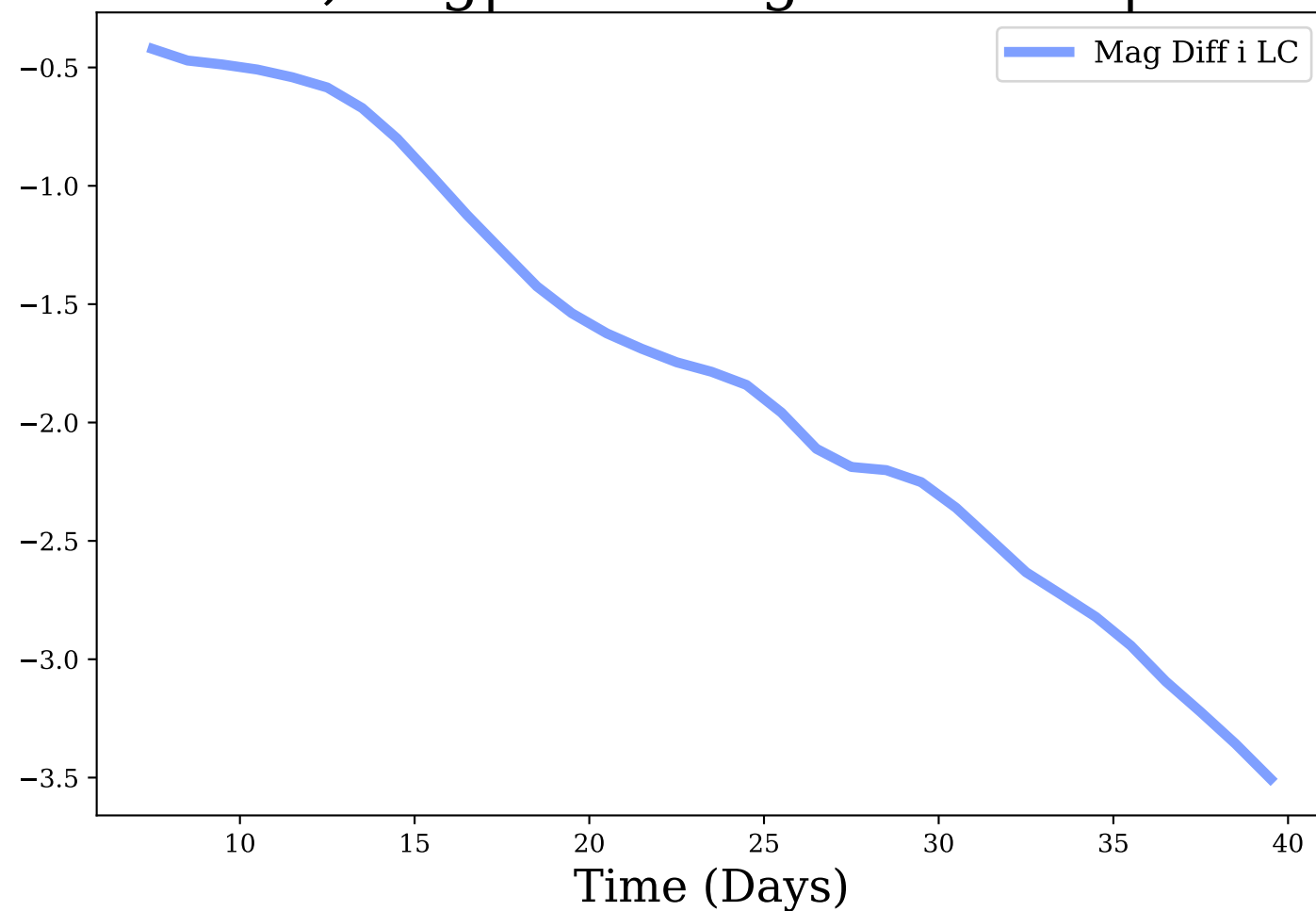
i-band, Avg|Max Mag Diff: -1.8 | 3.51
