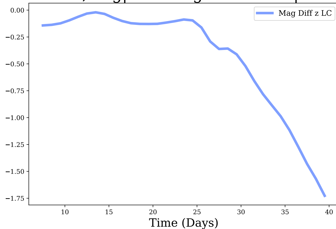
z-band, Avg|Max Mag Diff: -0.43 | 1.73
