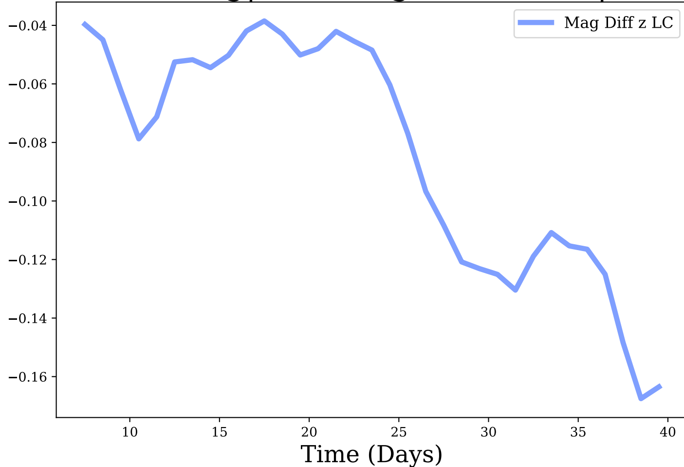
z-band, Avg|Max Mag Diff: -0.08 | 0.17
