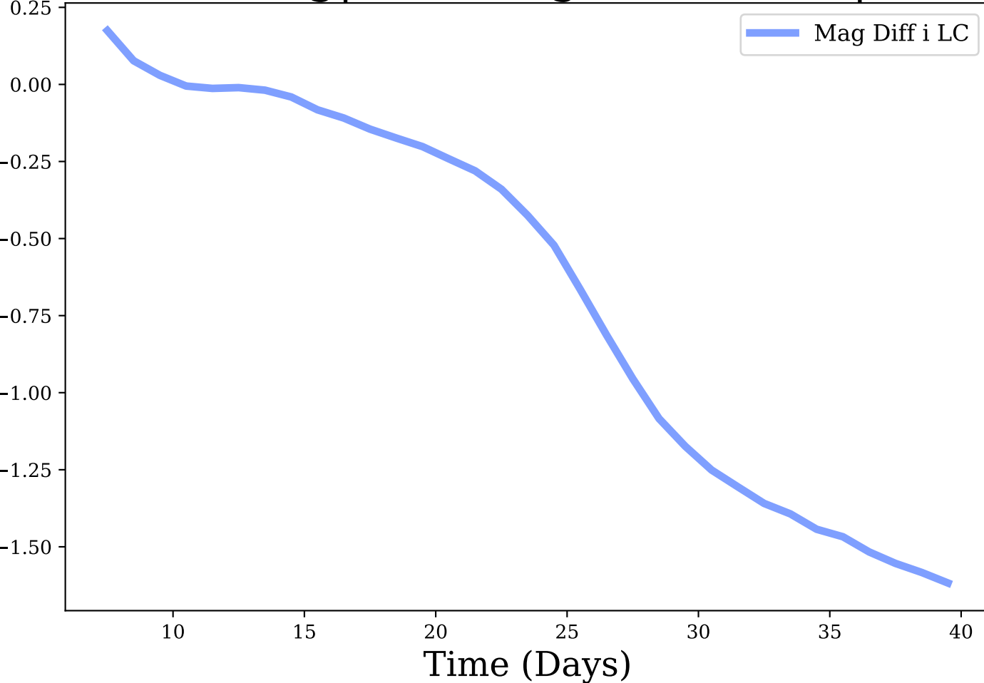
i-band, Avg|Max Mag Diff: -0.65 | 1.62
