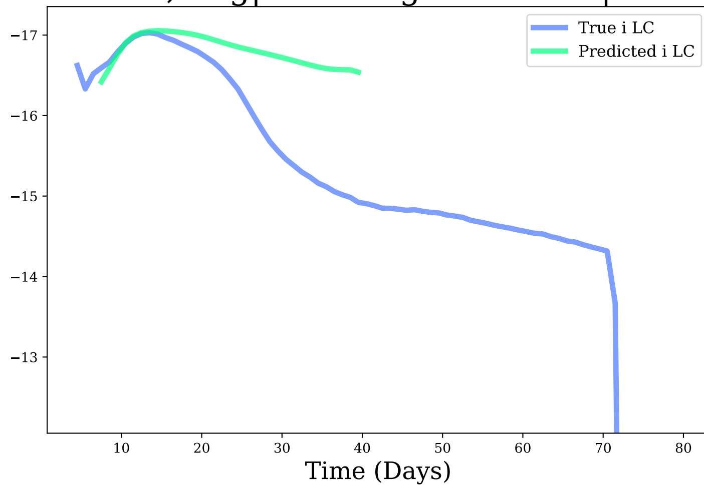
i-band, Avg|Max Mag Diff: 0.67 | 1.62
