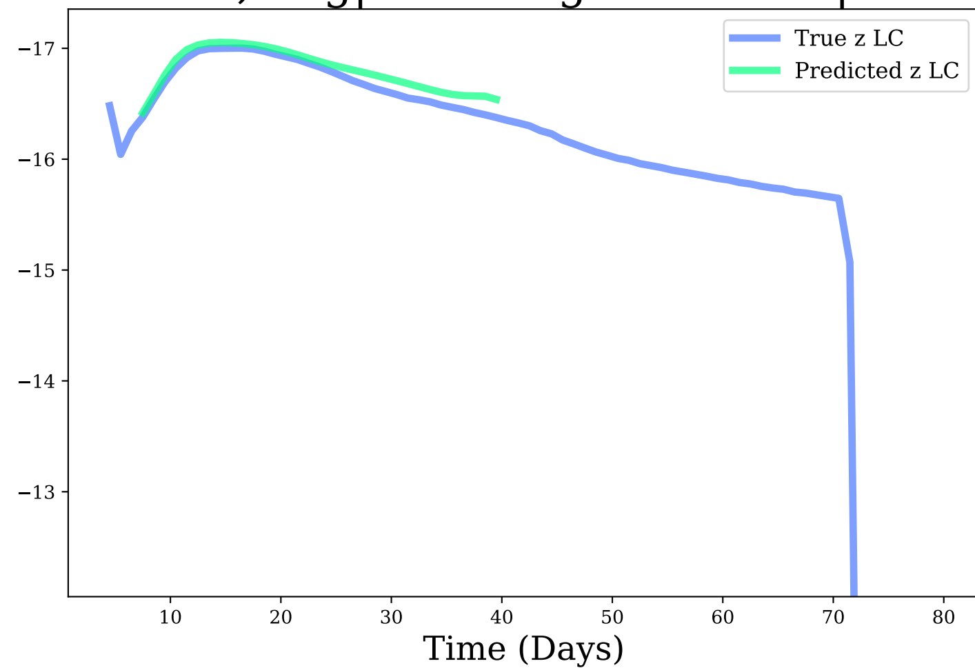
z-band, Avg|Max Mag Diff: 0.08 | 0.17
