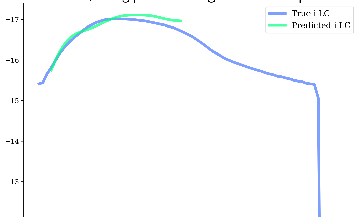
i-band, Avg|Max Mag Diff: 0.1 | 0.25
