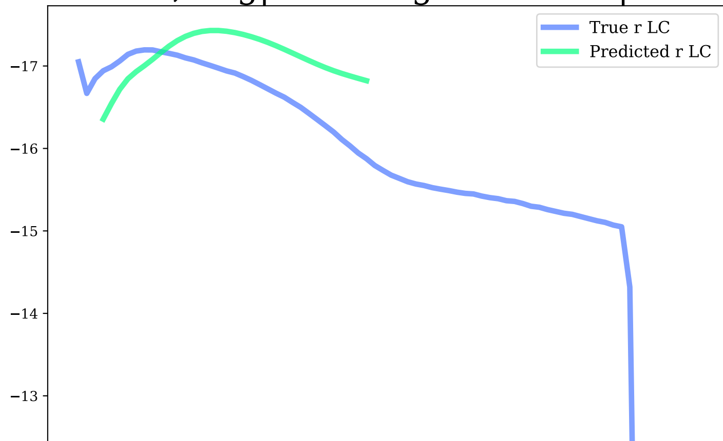
z-band, Avg|Max Mag Diff: 0.11 | 0.27
