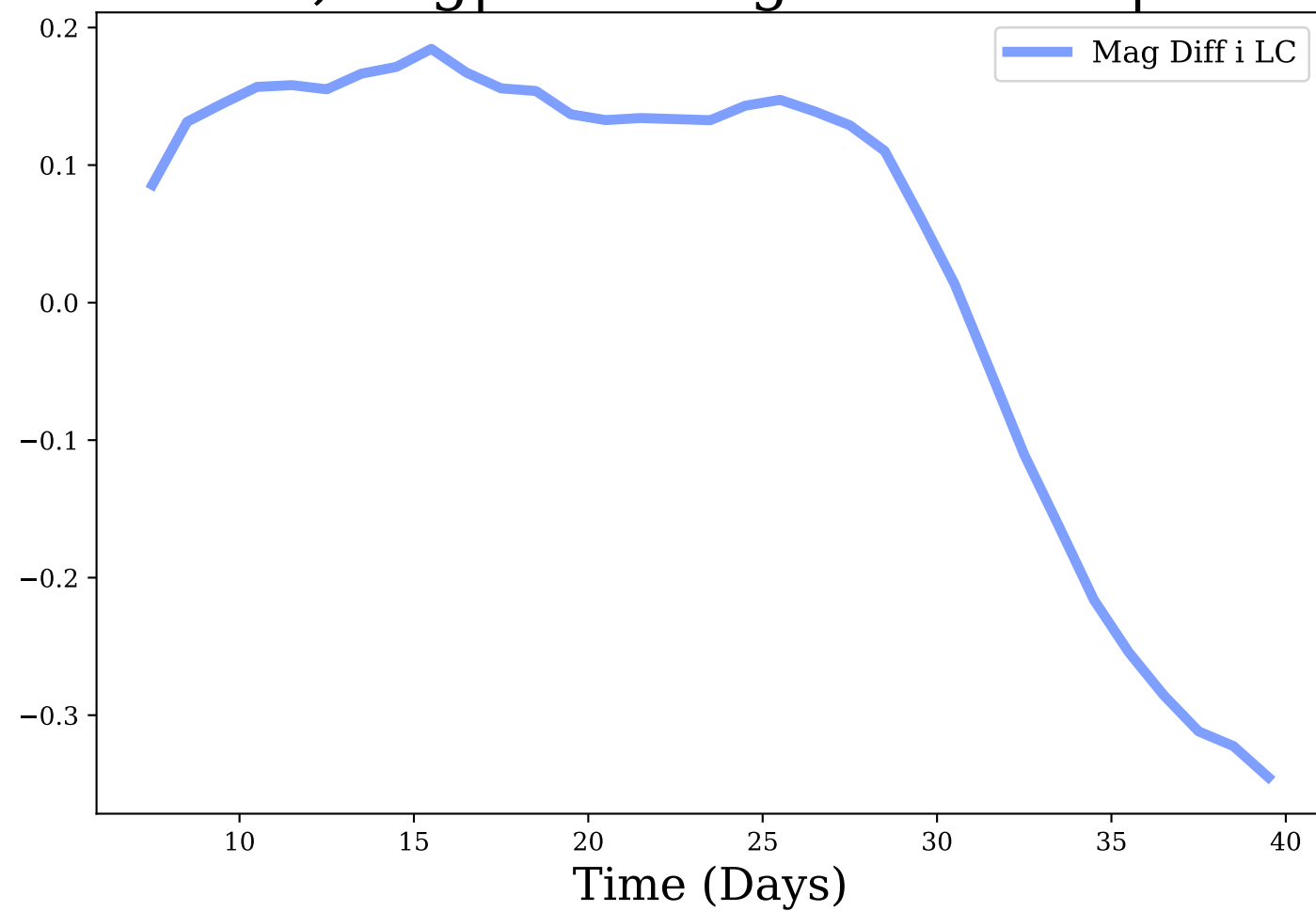
i-band, Avg|Max Mag Diff: 0.04 | 0.35
