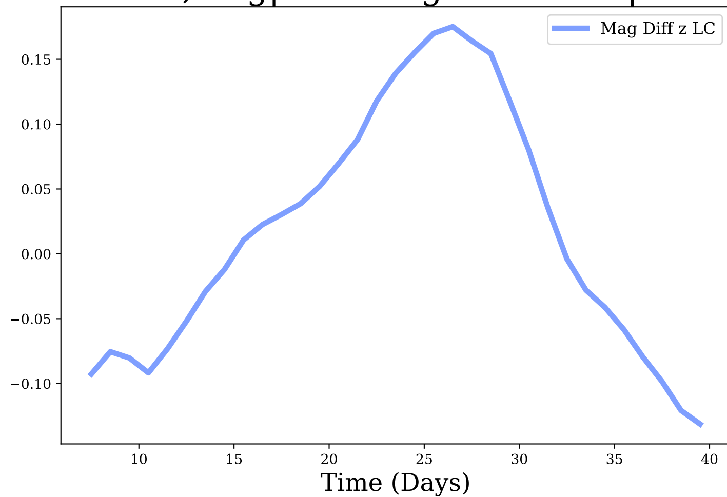
z-band, Avg|Max Mag Diff: 0.02 | 0.18
