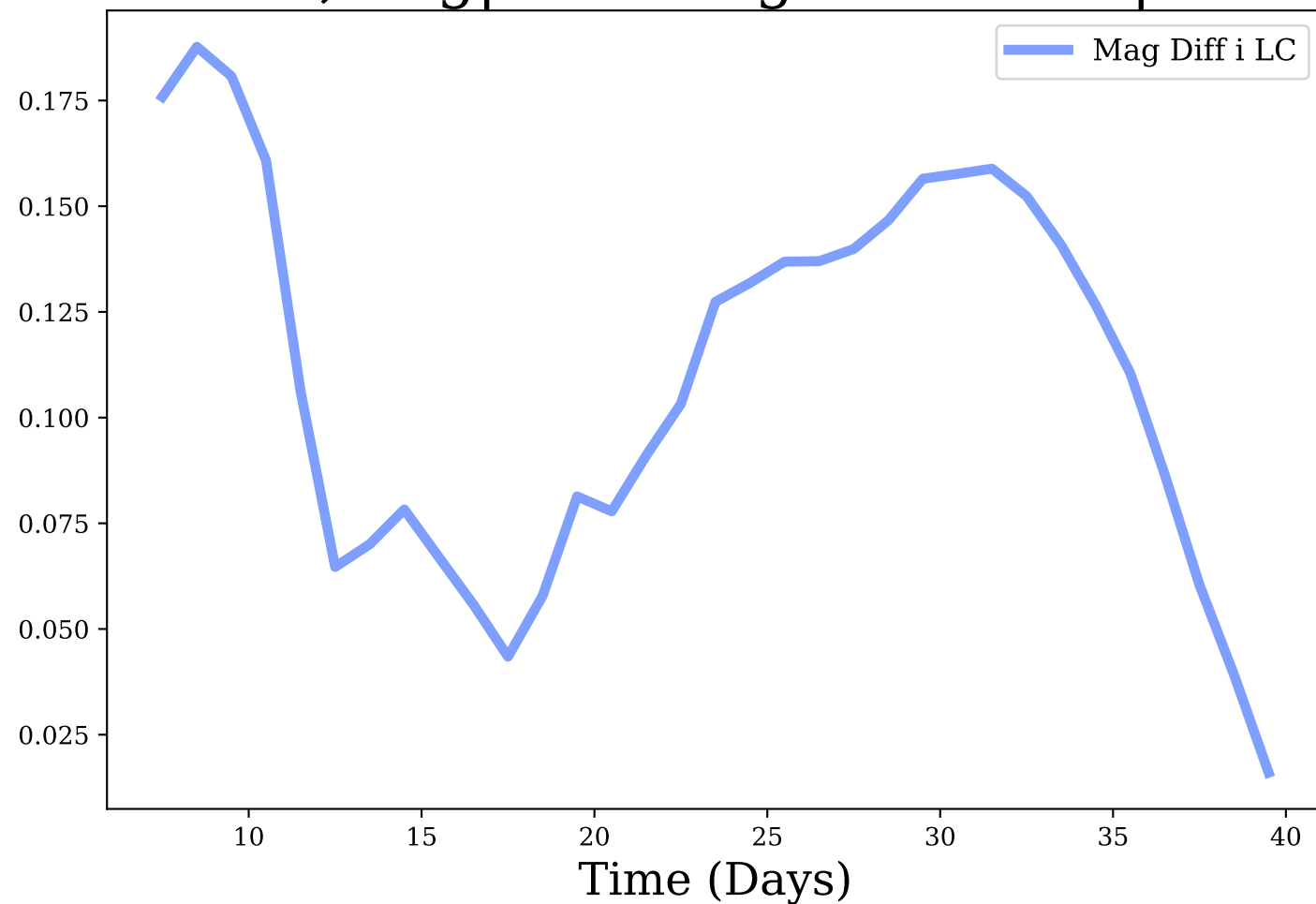
i-band, Avg|Max Mag Diff: 0.11 | 0.19
