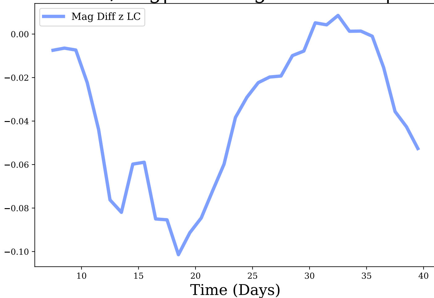
z-band, Avg|Max Mag Diff: -0.04 | 0.1
