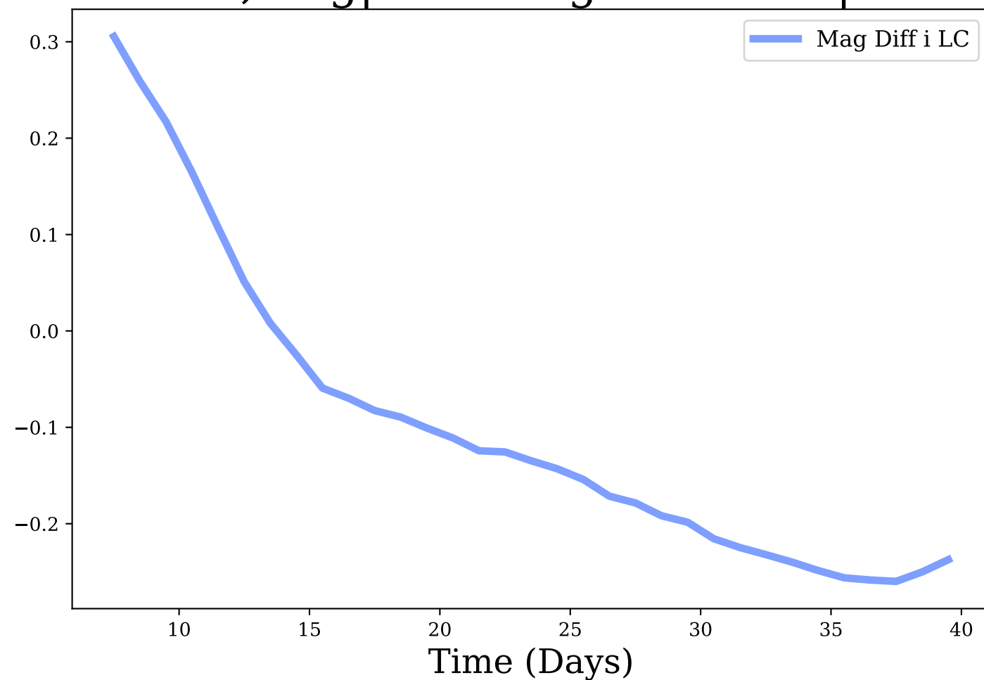
i-band, Avg|Max Mag Diff: -0.1 | 0.31
