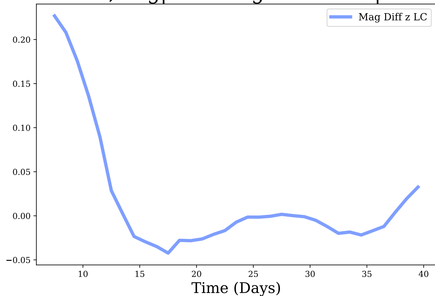
z-band, Avg|Max Mag Diff: 0.02 | 0.23
