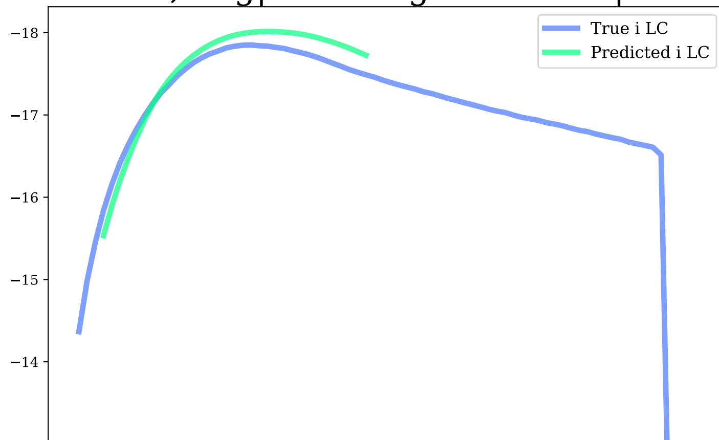
i-band, Avg|Max Mag Diff: 0.17 | 0.31
