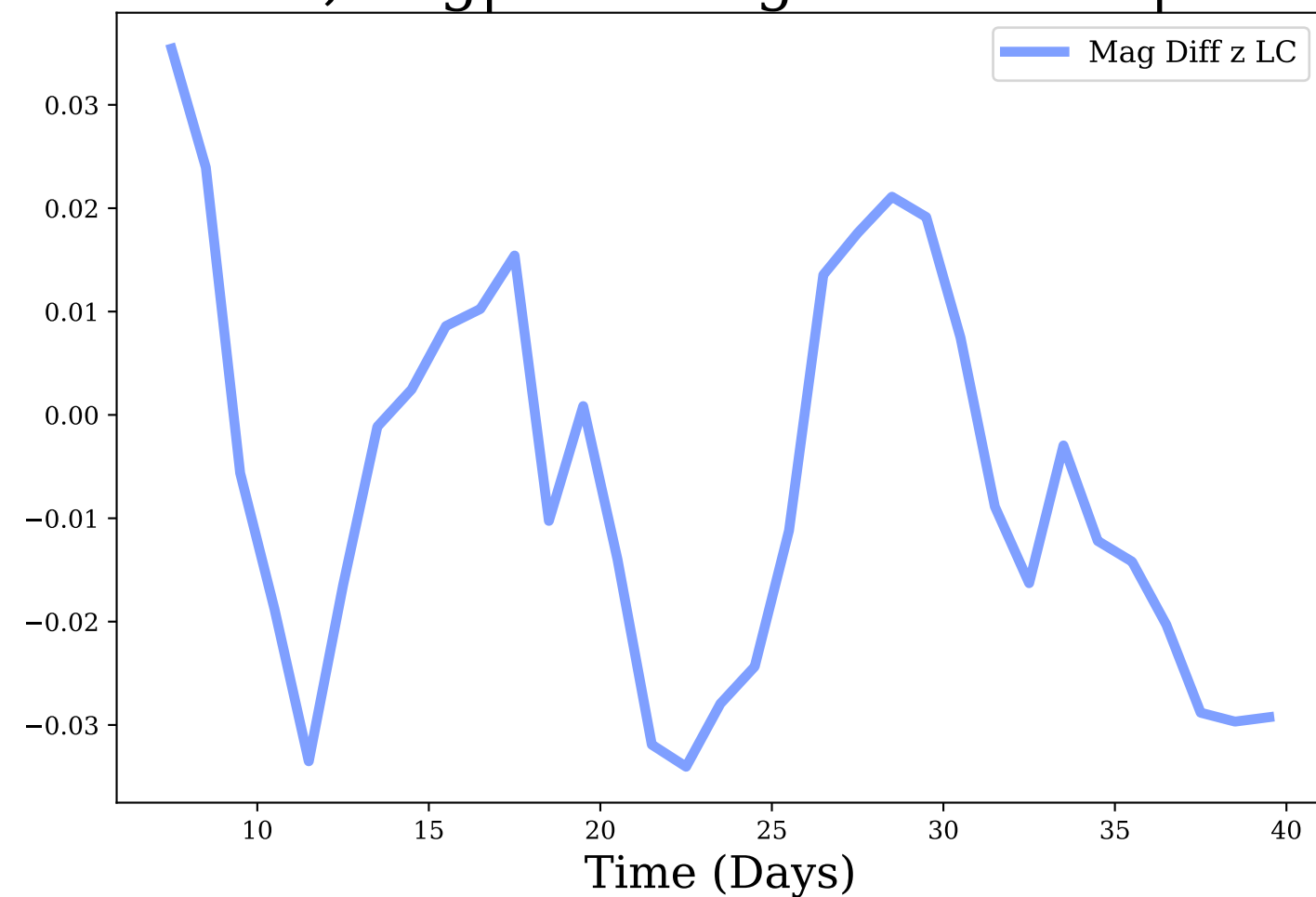
z-band, Avg|Max Mag Diff: -0.01 | 0.04
