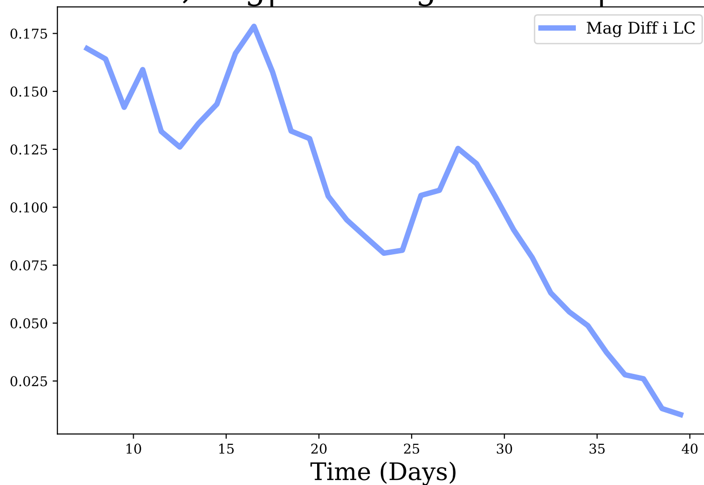
i-band, Avg|Max Mag Diff: 0.1 | 0.18
