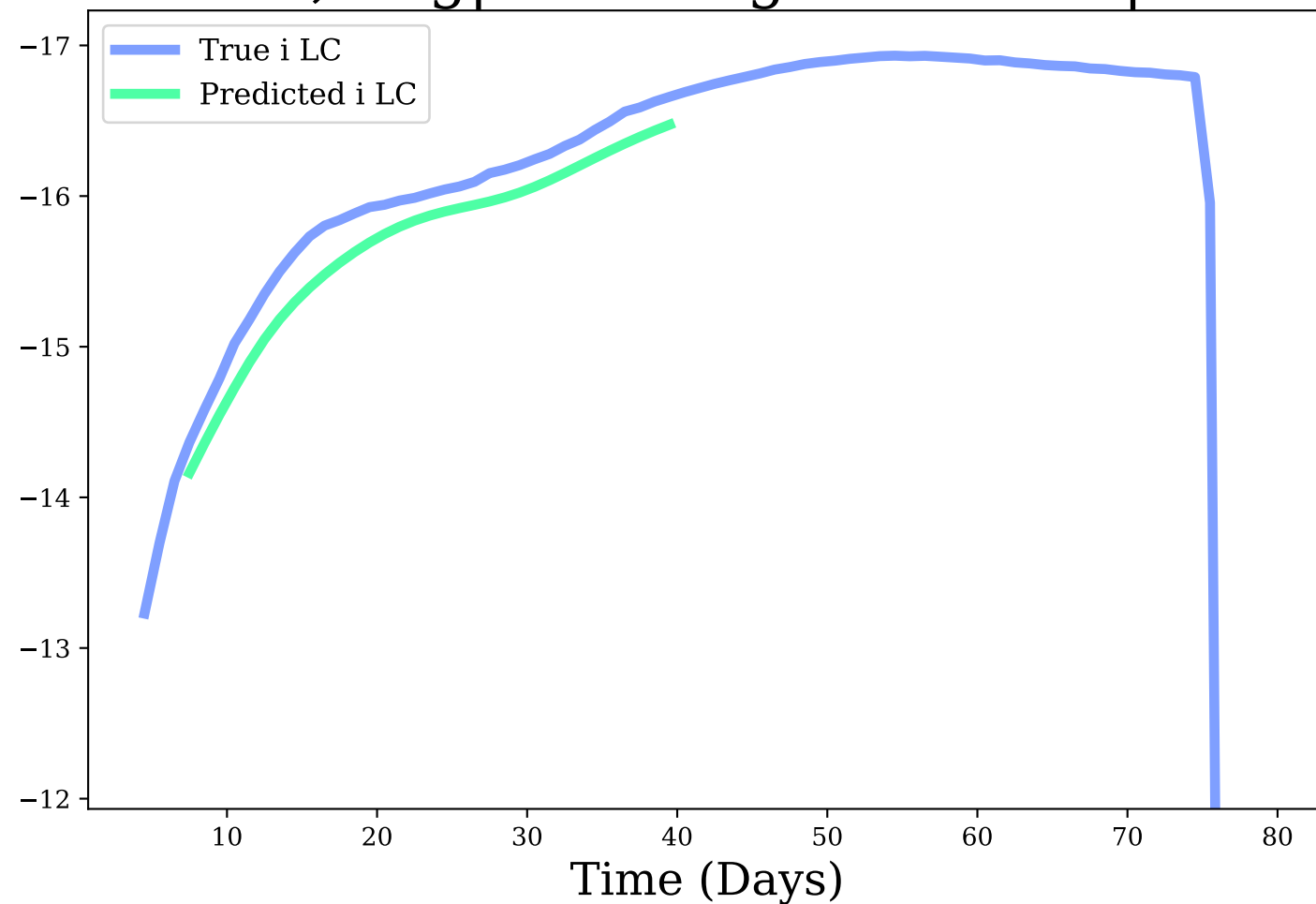
i-band, Avg|Max Mag Diff: 0.22 | 0.34
