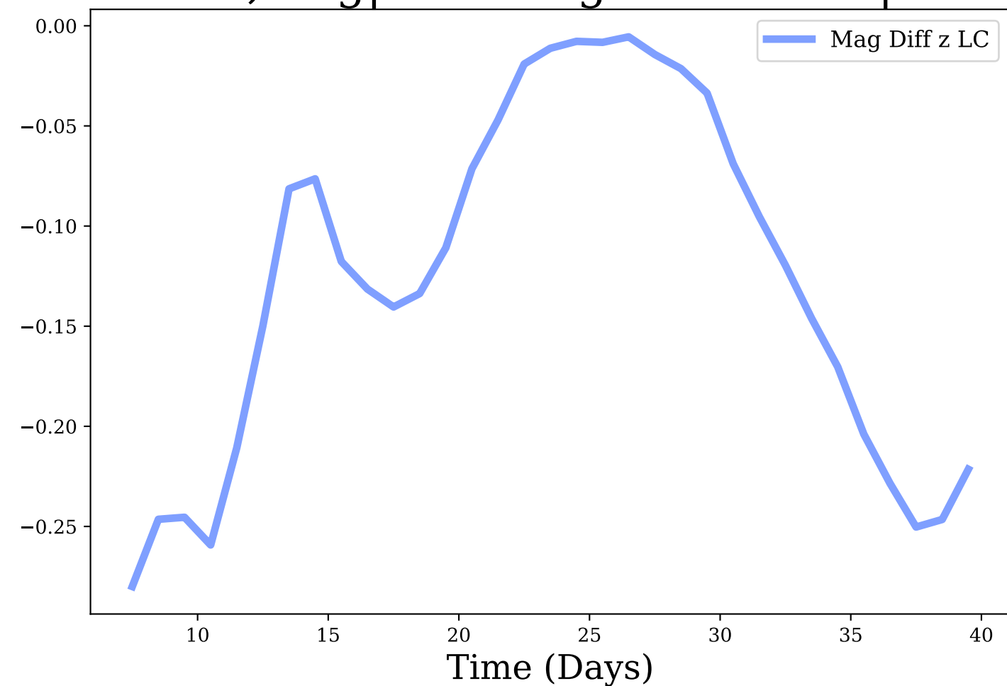
z-band, Avg|Max Mag Diff: -0.13 | 0.28
