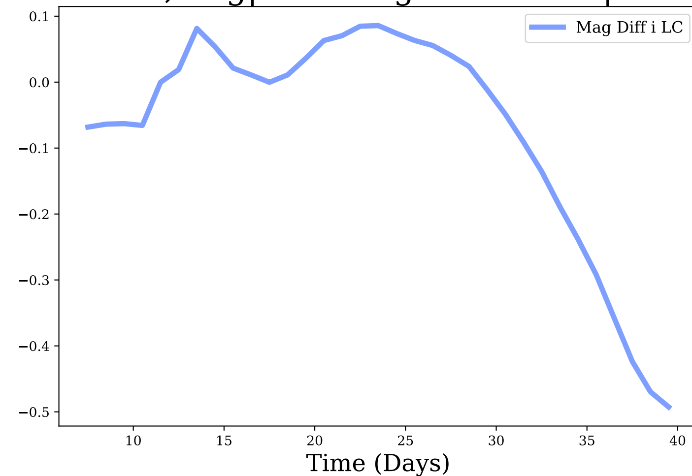
i-band, Avg|Max Mag Diff: -0.07 | 0.49
