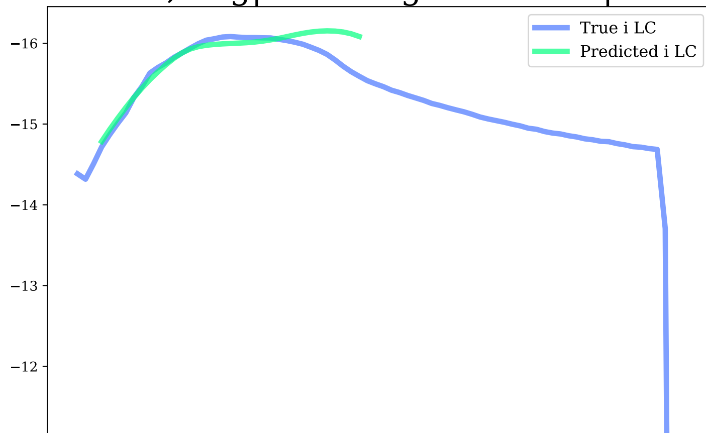
i-band, Avg|Max Mag Diff: 0.12 | 0.49
