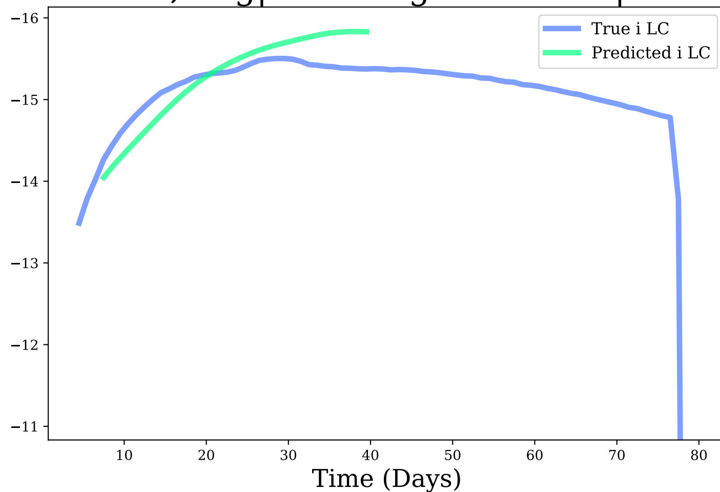
i-band, Avg|Max Mag Diff: 0.24 | 0.46
