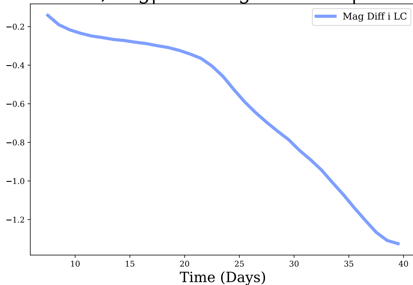
i-band, Avg|Max Mag Diff: -0.6 | 1.33
