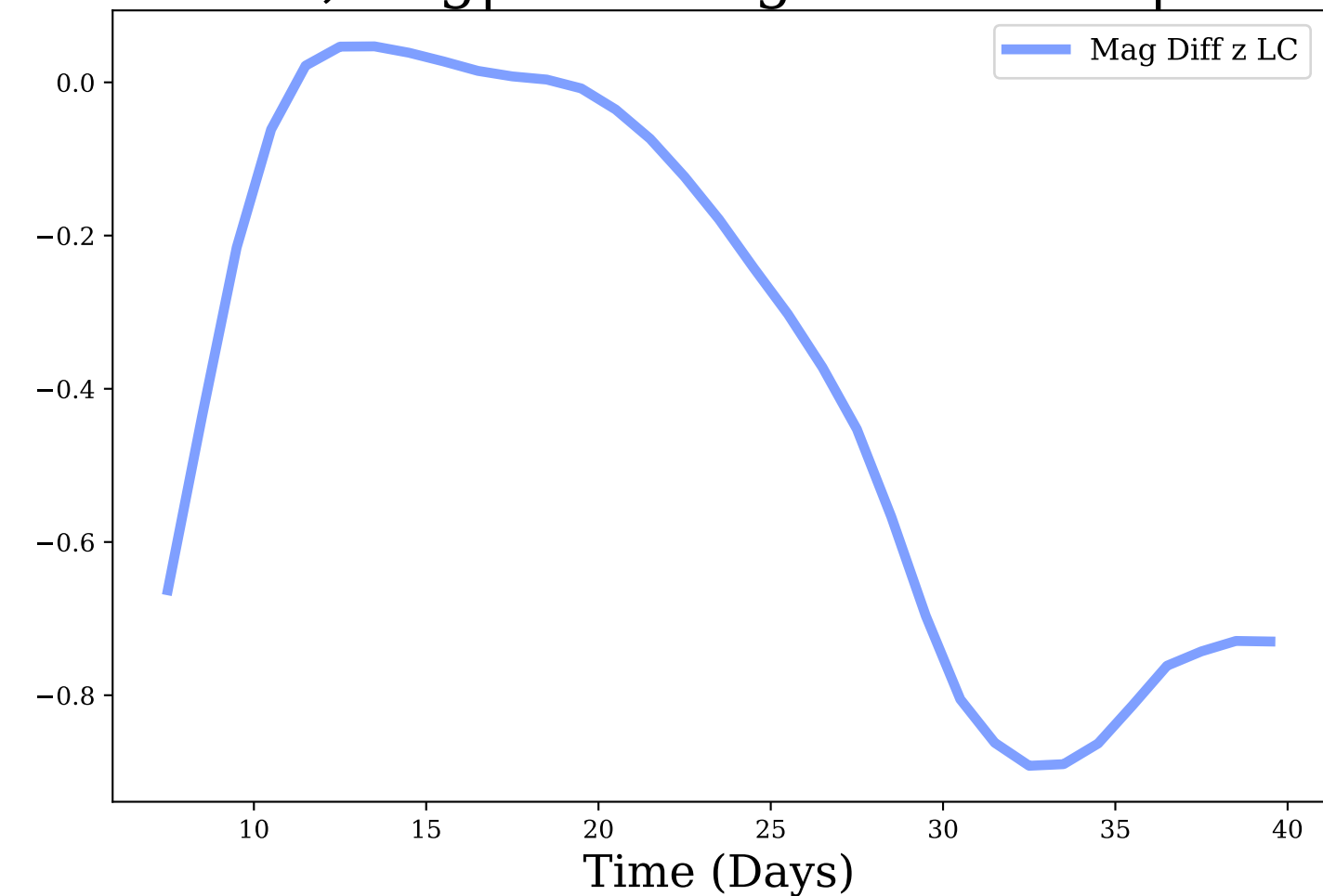
z-band, Avg|Max Mag Diff: -0.37 | 0.89
