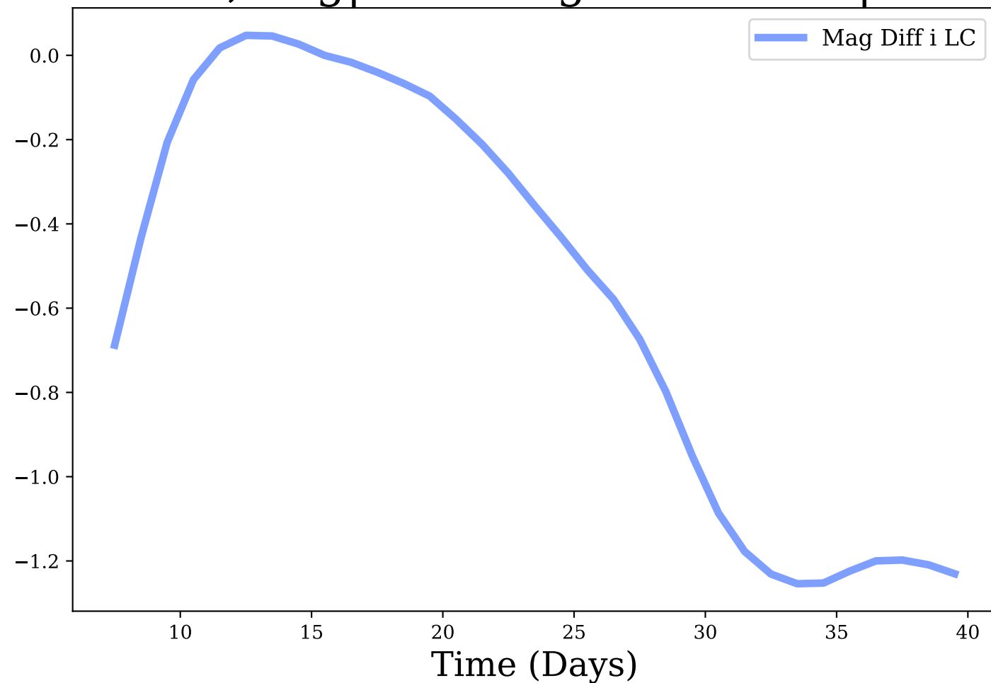
i-band, Avg|Max Mag Diff: -0.56 | 1.25
