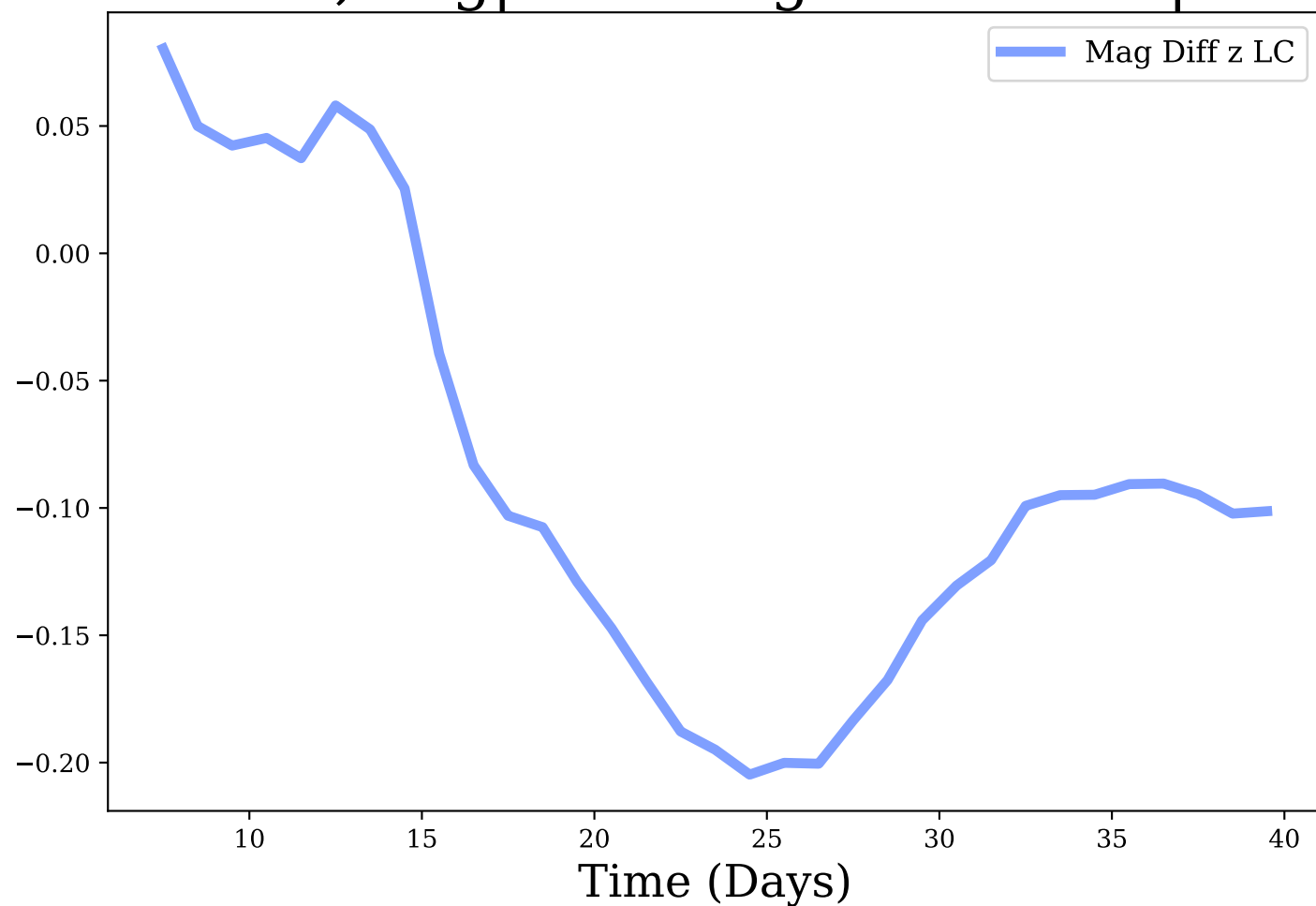
z-band, Avg|Max Mag Diff: -0.09 | 0.2
