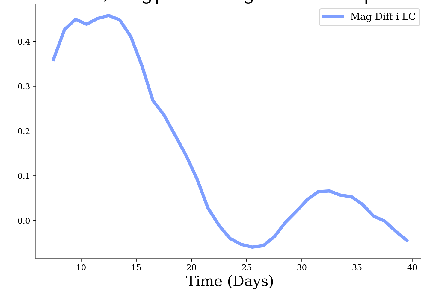
i-band, Avg|Max Mag Diff: 0.14 | 0.46
