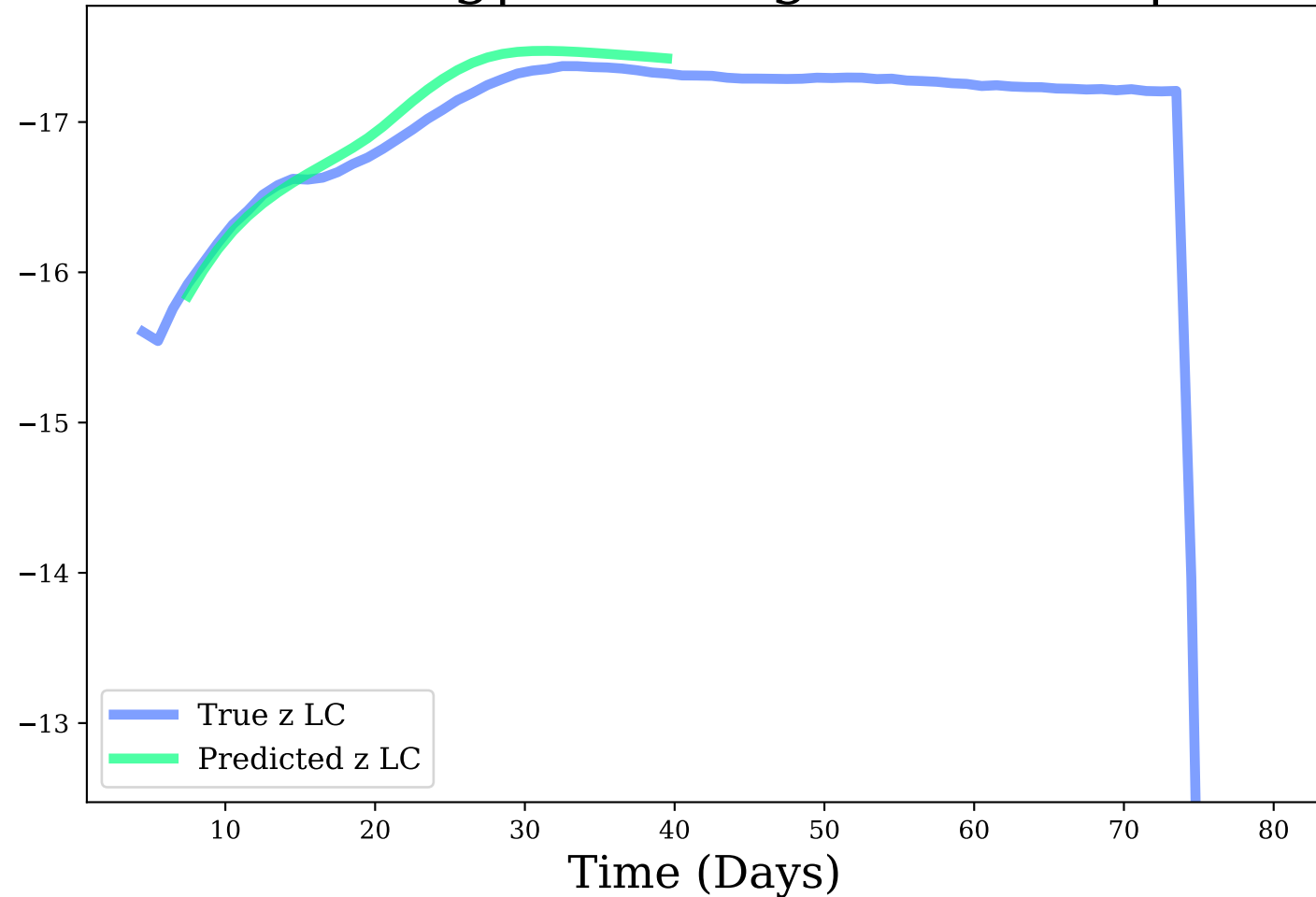
z-band, Avg|Max Mag Diff: 0.11 | 0.2
