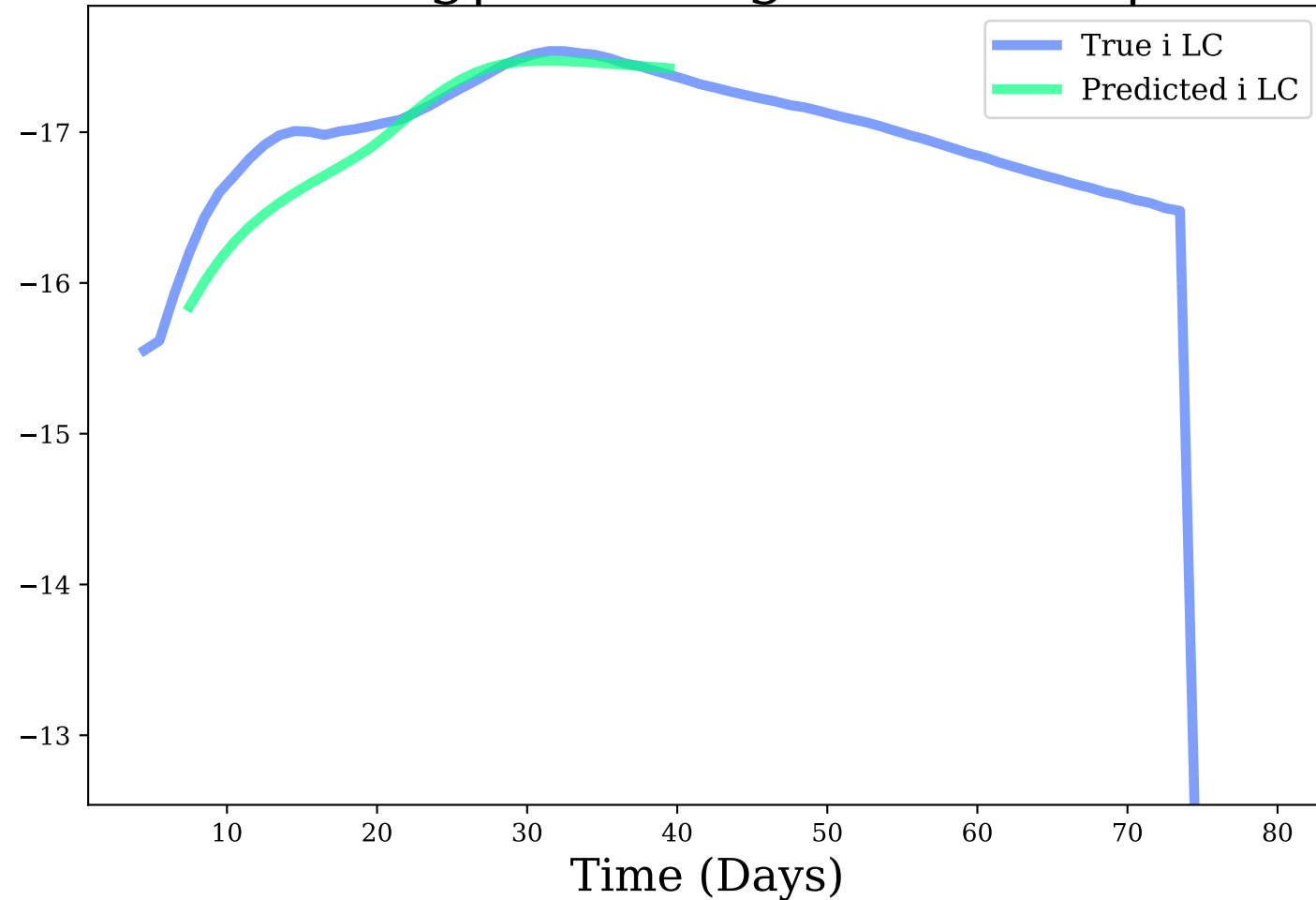
i-band, Avg|Max Mag Diff: 0.16 | 0.46
