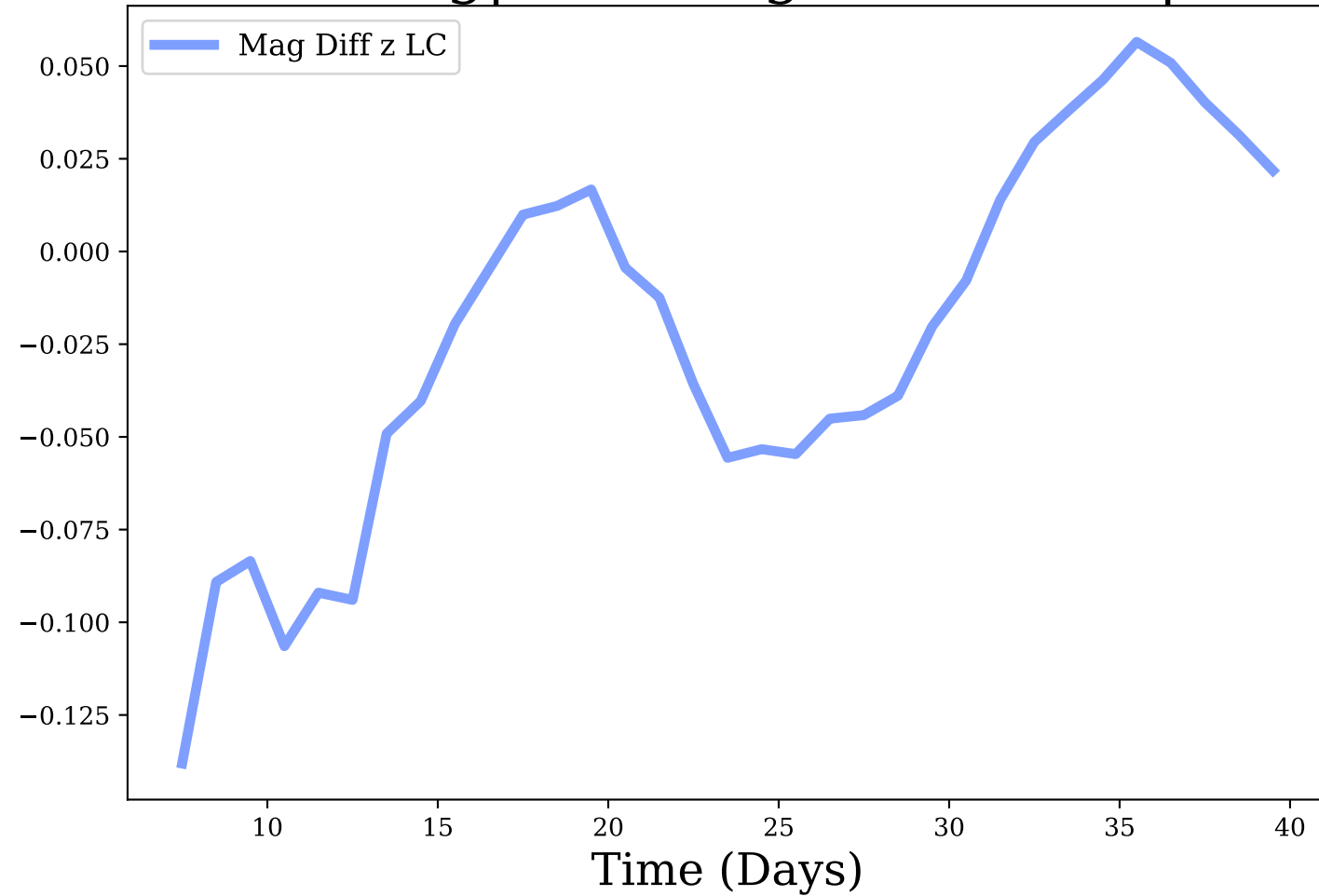
z-band, Avg|Max Mag Diff: -0.02 | 0.14
