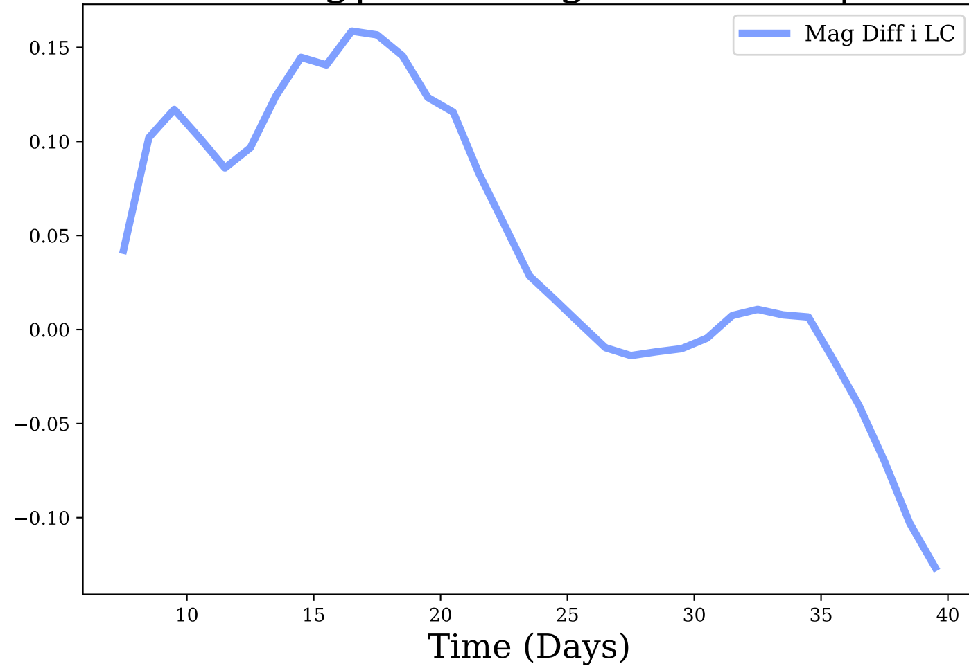
i-band, Avg|Max Mag Diff: 0.04 | 0.16
